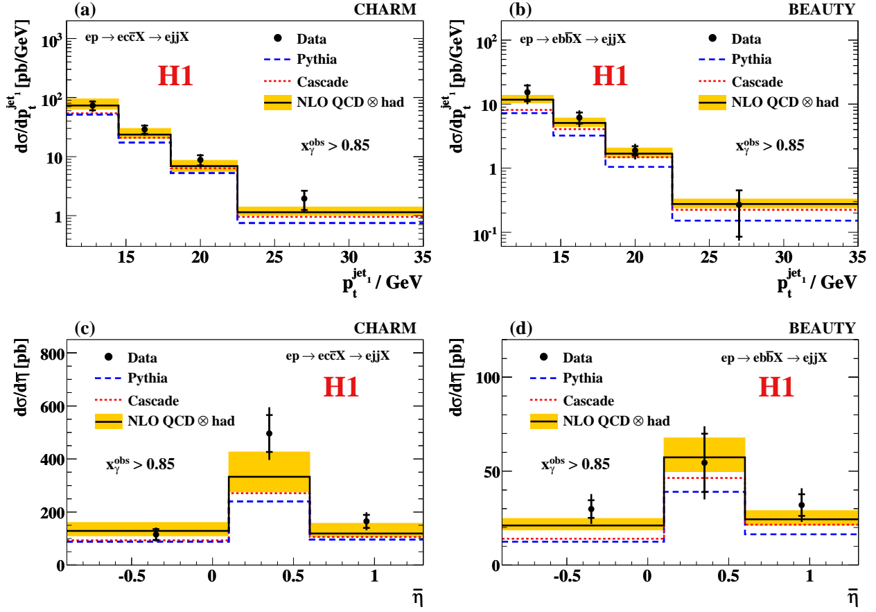
Figure 4: Differential charm and beauty photoproduction cross sections a,b) d\sigma/dp_t^{\text{jet}} and c,d) d\sigma/d\eta for the process ep \rightarrow e(c\bar{c} \text{ or } b\bar{b})X \rightarrow ejjX in the region x_\gamma^{\text{obs}} > 0.85 . The inner error bars indicate the statistical uncertainty and the outer error bars show the statistical and systematic errors added in quadrature. The solid lines indicate the prediction from a NLO QCD calculation, corrected for hadronisation effects, and the shaded band shows the estimated uncertainty. The absolute predictions from PYTHIA (dashed lines) and CASCADE (dotted lines) are also shown.
