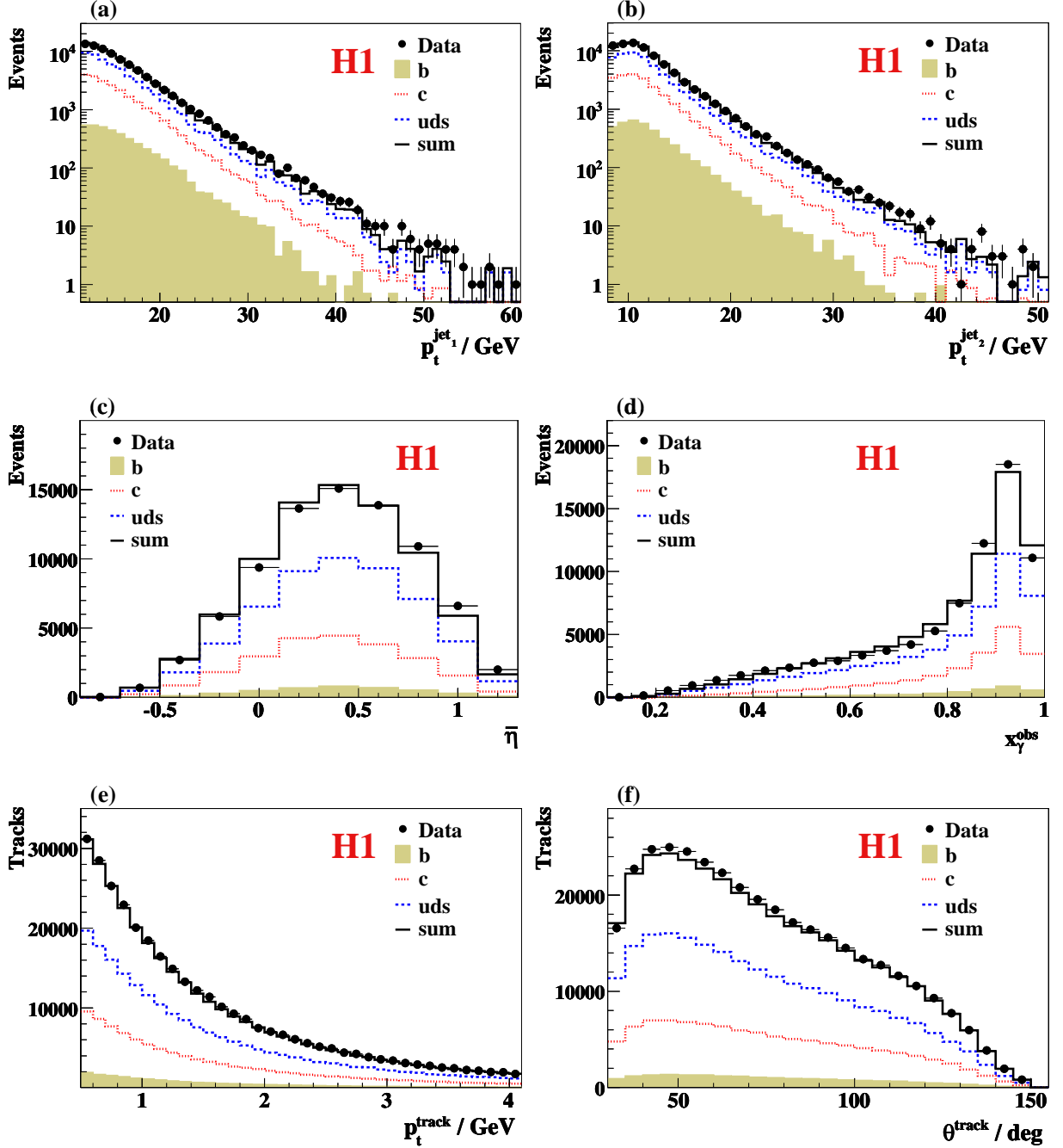
Figure 1: Distributions of a) the transverse momentum p_t^{\text{jet}1} of the leading jet, b) the transverse momentum p_t^{\text{jet}2} of the second jet, c) the mean pseudo-rapidity \bar{\eta} of the two jets, d) the observable x_\gamma^{\text{obs}} , e) the transverse momentum of the selected tracks and f) the polar angle of the selected tracks. The expectation from the PYTHIA Monte Carlo simulation is included in the figure, showing the contributions from the various quark flavours after applying the scale factors obtained from the fit to the subtracted significance distributions of the data (see section 4).
