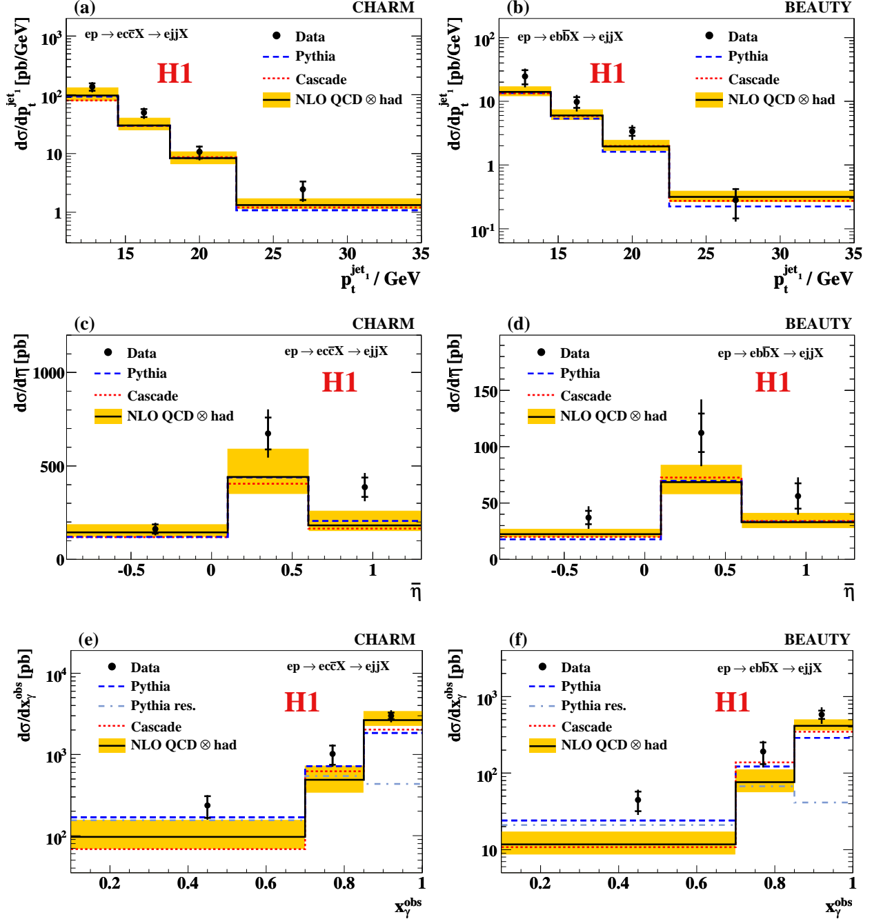
Figure 3: Differential charm and beauty photoproduction cross sections a,b) d\sigma/dp_t^{\text{jet}_1} , c,d) d\sigma/d\bar{\eta} and e,f) d\sigma/dx_\gamma^{\text{obs}} for the process ep \rightarrow e(c\bar{c} \text{ or } b\bar{b})X \rightarrow ejjX . The inner error bars indicate the statistical uncertainty and the outer error bars show the statistical and systematic errors added in quadrature. The solid lines indicate the prediction from a NLO QCD calculation, corrected for hadronisation effects, and the shaded band shows the estimated uncertainty. The absolute predictions from PYTHIA (dashed lines) and CASCADE (dotted lines) are also shown. The contribution from resolved processes in PYTHIA (dash-dotted lines) is depicted separately.
