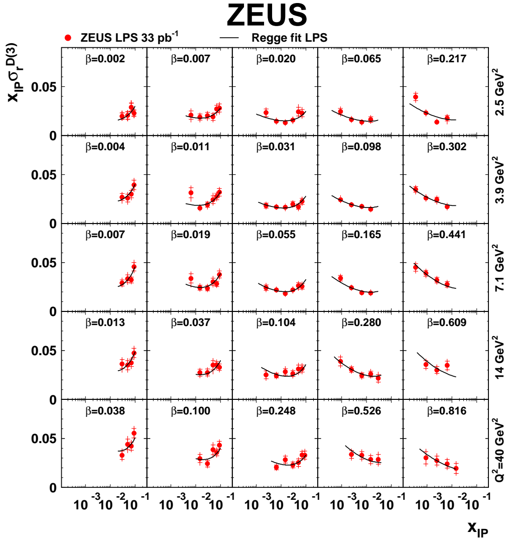
Figure 11: The reduced diffractive cross section multiplied by x_{\text{IP}} , x_{\text{IP}} \sigma_r^{D(3)} , obtained with the LPS method as a function of x_{\text{IP}} for different values of Q^2 and \beta . The lines are the result of the Regge fit described in Section 10.5. The inner error bars show the statistical uncertainties and the full bars indicate the statistical and the systematic uncertainties added in quadrature. The normalisation uncertainty of {}^{+11}_{-7}\% is not shown.
