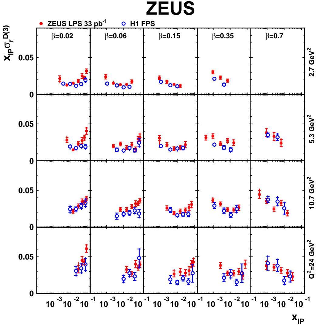
Figure 12: The reduced diffractive cross section multiplied by x_{\mathbb{P}}, x_{\mathbb{P}}\sigma_r^{D(3)} , obtained with the LPS method (dots) as a function of x_{\mathbb{P}} for different values of Q^2 and \beta compared with the results obtained with the H1 Forward Proton Spectrometer (open circles). The inner error bars show the statistical uncertainties and the full bars indicate the statistical and the systematic uncertainties added in quadrature. The normalisation uncertainty of ^{+11}_{-7}\% of the ZEUS data is not shown, nor is that of the H1 data ( \pm 10\% ).
