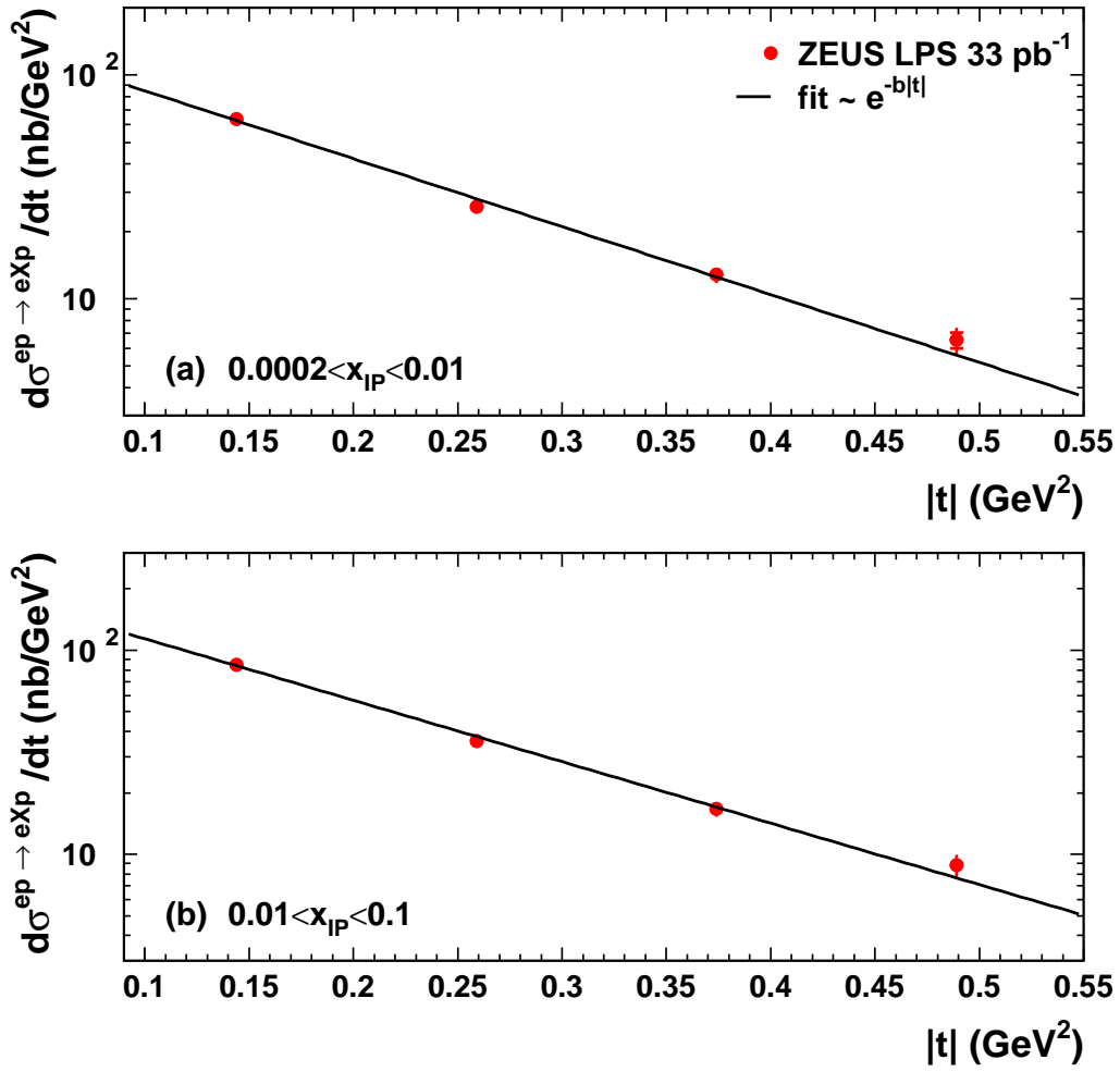
Figure 6: The differential cross-section d\sigma^{ep \rightarrow eXp}/dt for (a) 0.0002 < x_{IP} < 0.01 and (b) 0.01 < x_{IP} < 0.1 . The lines show the results of fits with the function d\sigma^{ep \rightarrow eXp}/dt \propto e^{-b|t|} . The inner error bars show the statistical uncertainties and the full bars indicate the statistical and the systematic uncertainties added in quadrature. The normalisation uncertainty of \pm 7\% is not shown.
