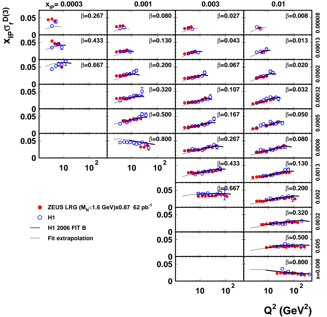
Figure 18: The reduced diffractive cross section multiplied by x_P , x_P \sigma_r^{D(3)} , obtained with the LRG method (dots) as a function of Q^2 for different \beta and x_P values compared with the H1 results (open circles), also obtained with the LRG method. The lines represent the expectation based on the diffractive parton distribution functions “H1 2006 fit B”. The inner error bars show the statistical uncertainties and the full bars indicate the statistical and the systematic uncertainties added in quadrature. The ZEUS data are normalised to the H1 data.
