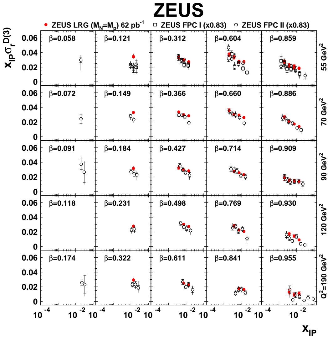
Figure 20: The reduced diffractive cross section multiplied by x_{IP} , x_{IP} \sigma_r^{D(3)} , obtained with the LRG method (dots) as a function of x_{IP} for different values of Q^2 and \beta at high Q^2 . Other details as in caption for Fig. 19.
