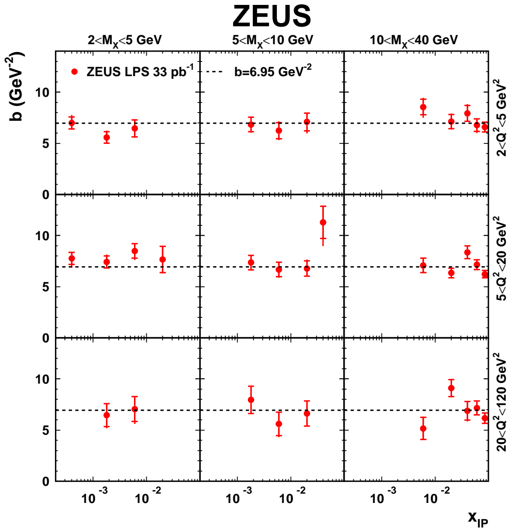
Figure 7: The value of the exponential-slope parameter b of the differential cross-section d\sigma^{ep \rightarrow eXp}/dt \propto e^{-b|t|} as a function of x_{\mathbb{P}} in bins of Q^2 and M_X . The dashed line corresponds to the value of b = 6.95 \text{ GeV}^{-2} , the average t -slope over the measured region. The inner error bars show the statistical uncertainties and the full bars indicate the statistical and the systematic uncertainties added in quadrature.
