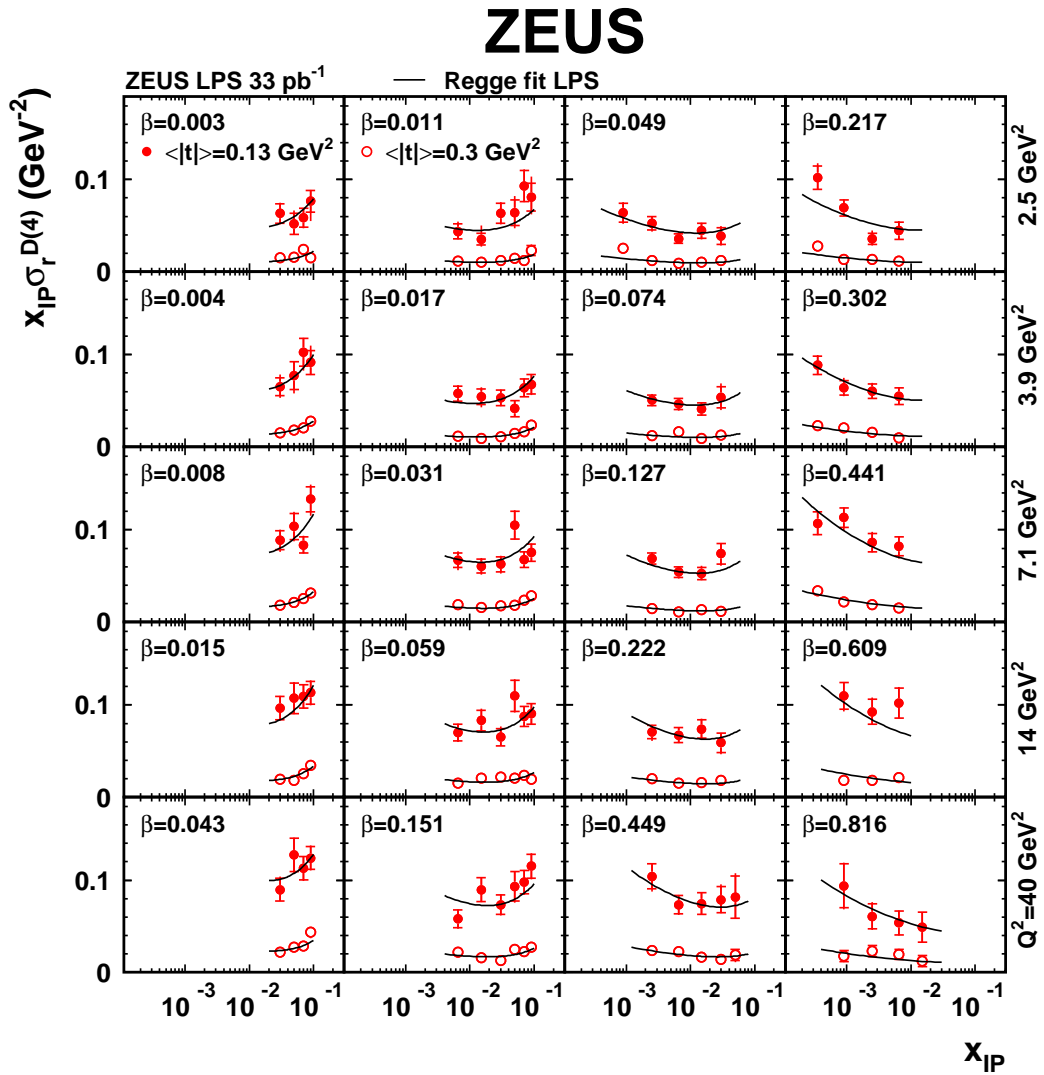
Figure 10: The reduced diffractive cross section multiplied by x_P , x_P \sigma_r^{D(4)} , obtained with the LPS method in two t bins as a function of x_P for different values of Q^2 and \beta . The lines are the result of the Regge fit described in Section 10.5. The inner error bars show the statistical uncertainties and the full bars indicate the statistical and the systematic uncertainties added in quadrature. The normalisation uncertainty of \pm 7\% is not shown.
