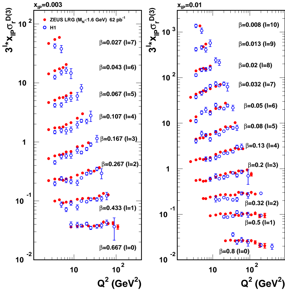
Figure 17: The reduced diffractive cross section multiplied by x_{\mathbb{P}} , x_{\mathbb{P}}\sigma_r^{D(3)} , obtained with the LRG method (dots) at x_{\mathbb{P}} = 0.003 and x_{\mathbb{P}} = 0.01 as a function of Q^2 for different \beta values compared with the H1 results (open circles), also obtained with the LRG method. Other details as in caption for Fig. 16.
