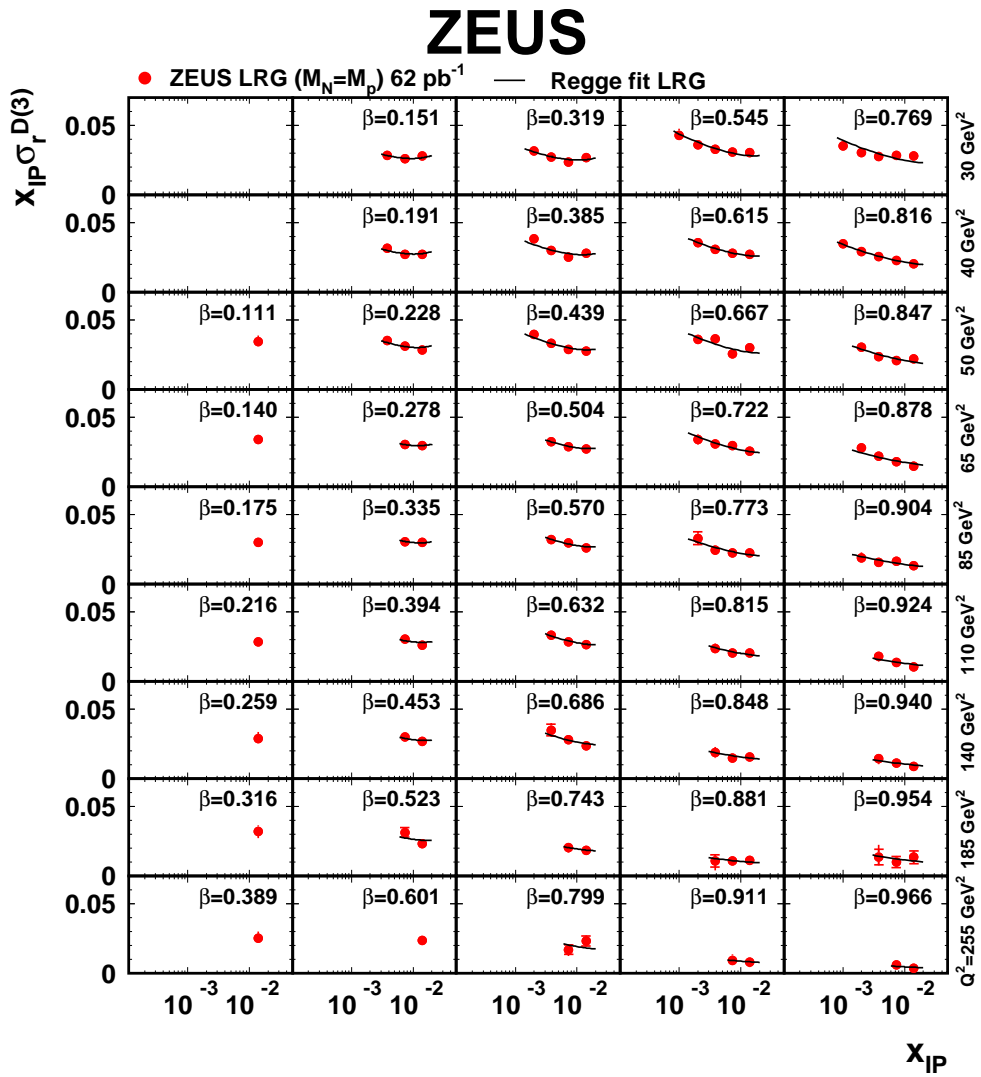
Figure 14: The reduced diffractive cross section multiplied by x_{\mathbb{P}} , x_{\mathbb{P}} \sigma_r^{D(3)} , obtained with the LRG method as a function of x_{\mathbb{P}} for different values of Q^2 and \beta at high Q^2 values. Other details as in caption for Fig. 13.
