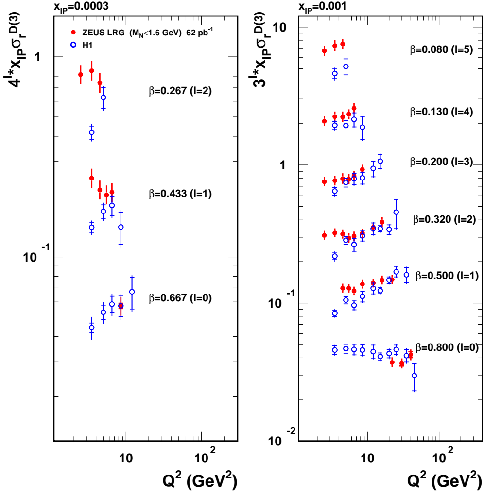
Figure 16: The reduced diffractive cross section multiplied by x_{\mathbb{P}} , x_{\mathbb{P}}\sigma_r^{D(3)} , obtained with the LRG method (dots) at x_{\mathbb{P}} = 0.0003 and x_{\mathbb{P}} = 0.001 as a function of Q^2 for different \beta values compared with the H1 results (open circles), also obtained with the LRG method. The inner error bars show the statistical uncertainties and the full bars indicate the statistical and the systematic uncertainties added in quadrature. The ZEUS data are corrected to M_N < 1.6 GeV as described in Section 10.4. The 8% uncertainty on the correction is not shown, nor is the 7% relative normalisation uncertainty between the ZEUS and H1 data sets.
