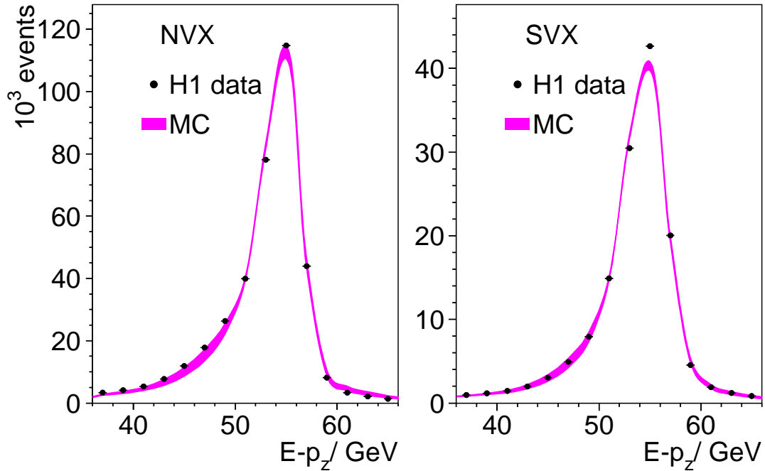
Figure 18: E-p_z distribution for the data and the MC simulation in the NVX and the SVX analyses. The bands include the statistical uncertainty of the simulation and the effect of a \pm 0.5 GeV variation of the SpaCal hadronic final state contribution.
