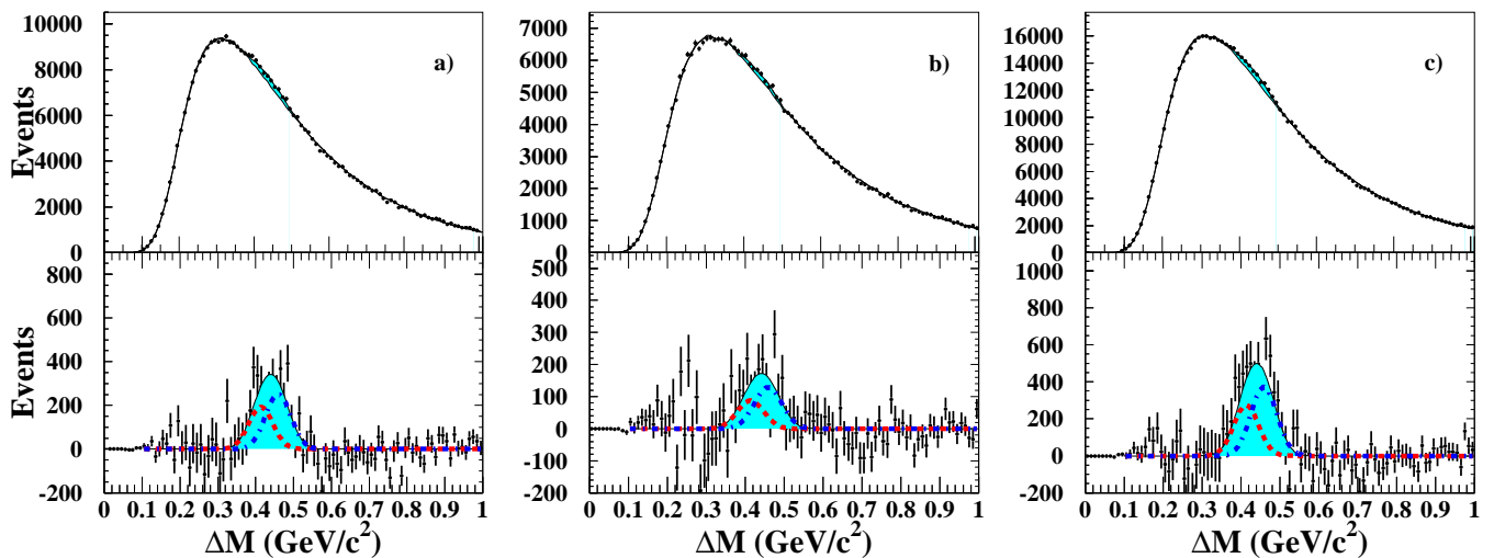
FIG. 6: \Delta M spectra in the electron channel for C (a), W (b) and full sample (c). The Ti spectrum is not shown due to the low statistics. The bin width is 10\text{MeV}/c^2 . In the background subtracted spectra the broken curves are the fitted \chi_{c1} and \chi_{c2} states.
