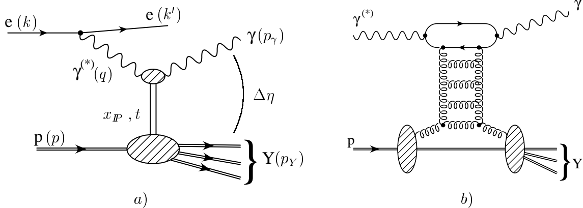
Figure 1: a) Schematic illustration of the ep \rightarrow e\gamma Y process. b) Illustration of the \gamma^{(*)}p \rightarrow \gamma Y process in a LLA BFKL approach.
