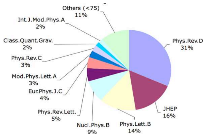
Figure 1. Journals favoured by HEP scientists in 2006. Data from the SPIRES database. Journals that attracted less than 75 HEP articles are grouped in the slice named “Others”.
