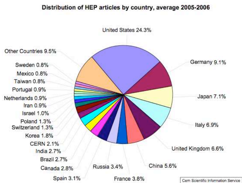
Figure 2. Contributions by country to the HEP scientific literature published in the largest journals in the field. Co-authorship is taken into account on a pro-rata basis, assigning fractions of each article to the countries in which the authors are affiliated. This study is based on over 11’000 articles published in the years 2005 and 2006. Countries with individual contributions less than 0.8% are aggregated in the “Other countries” category 14 .
