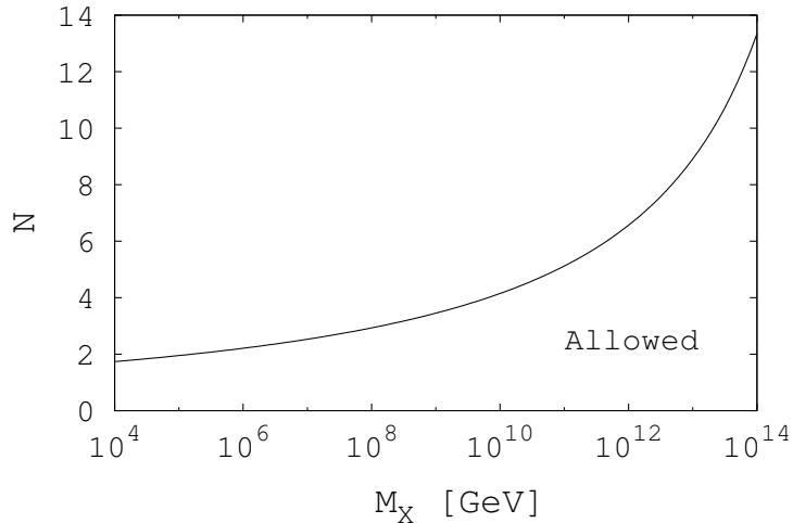
FIG. 1: The region for the messenger parameters M_X and N allowed by the positivity constraint on the right-handed scalar lepton mass in the minimal supersymmetric SM.
