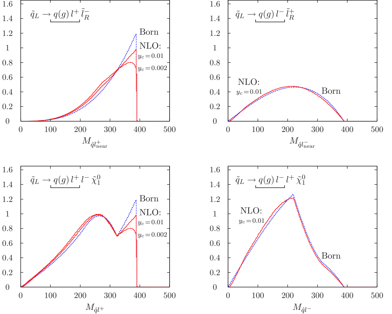
Figure 3: The [\hat{q}l^{\pm}] invariant mass distributions for positively (left panels) and negatively (right panels) charged leptons is shown at SPS1a' [specifically for \tilde{u}_L masses and first and second generation leptons with vanishing masses]. The upper panels include only “near” leptons while the lower panels display the sum of “near” and “far” leptons. The NLO predictions are represented by the solid lines for y_c = 0.01 and 0.002 , the Born result [approximately equivalent to NLO with y_c \gtrsim 0.05 ] by the dashed line.
