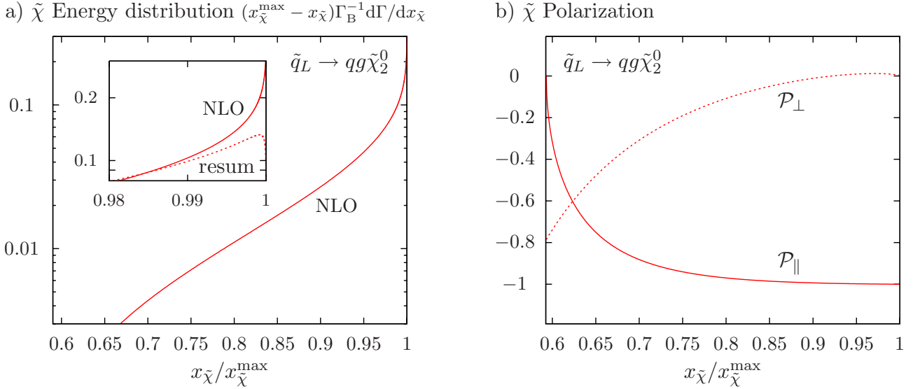
Figure 2: (a) The differential decay rate for \tilde{q}_L \rightarrow qg\tilde{\chi}_2^0 as a function of the \tilde{\chi}_2^0 energy x_{\tilde{\chi}} at the benchmark point SPS1a' ( M_{\tilde{\chi}}/M_{\tilde{q}} = 0.329 ). The curve labeled “resum” shows the damping near x_{\tilde{\chi}}^{\max} from multiple gluon radiation according to Eq. (2.5). (b) The longitudinal and transverse polarization of the neutralino \tilde{\chi}_2^0 .
