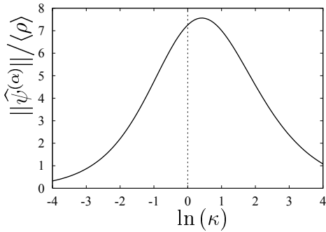
Figure 5: Colour zero modes \lambda_\alpha
