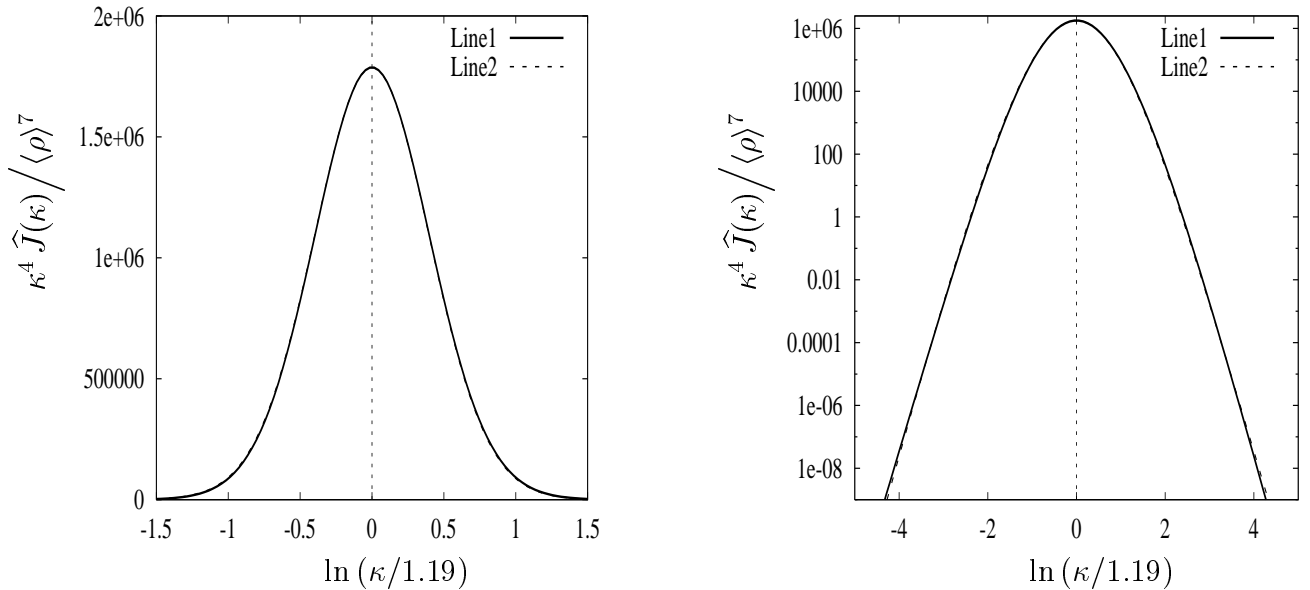
Figure 7: (Left): Total zero mode contribution \kappa^5 \widehat{J}(\kappa)/\langle\rho\rangle^7 times 1/\kappa on the sphere, as relevant for the instanton size distribution d(\rho\mu_r, \alpha_s) in Eq. (20). As abscissa, we use \ln(\kappa/1.19) = \ln(\rho/(1.19\langle\rho\rangle)) to make small deviations from a perfect size inversion symmetry for \kappa/1.19 \leftrightarrow 1.19/\kappa self-evident. Line1 and Line2 display the results versus \kappa/1.19 and 1.19/\kappa , respectively. (Right): Same plot, but using a logarithmic ordinate, to demonstrate the high degree of inversion symmetry over fourteen orders of magnitude, with Line1 and Line2 being visually indistinguishable!
