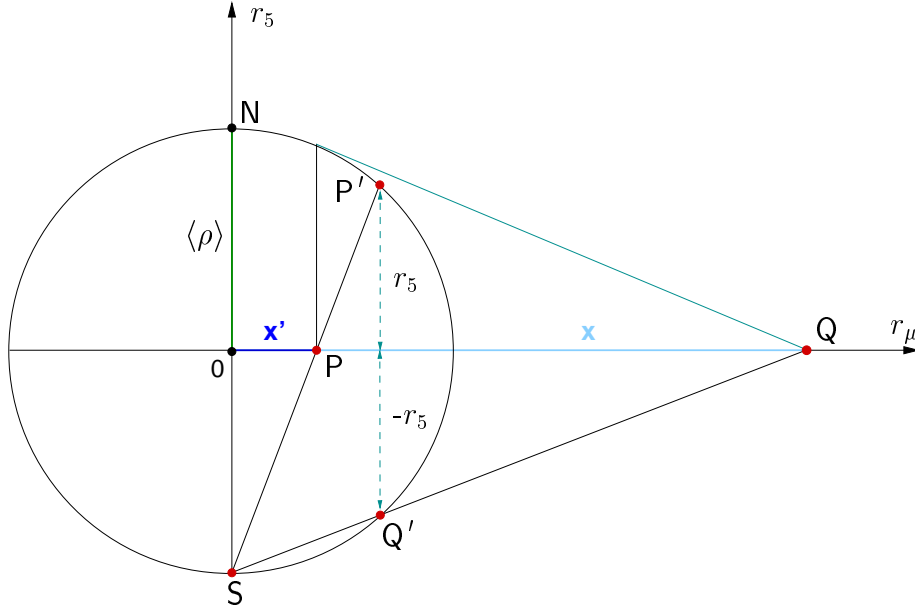
Figure 2: Relation between inversion and stereographic projection: The points P and Q define the two distances x and x' , which are related by the condition of inversion, x^2 x'^2 = \langle \rho \rangle^4 . As a consequence, the projected points P' and Q' differ only in the sign of the coordinate r_5 . An inversion leads to an exchange of the northern and southern hemisphere.
