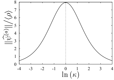
Figure 4: Colour zero modes \lambda_a
