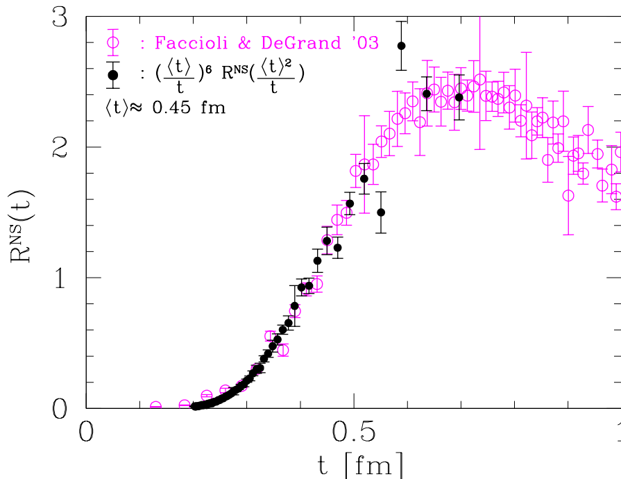
Figure 8: Alternative test of conformal (space-) time inversion symmetry for t \rightarrow \langle t \rangle^2/t , according to Eqs. (50, 52) for the chirality-flip correlator R^{\text{NS}}(t) , using directly (quenched) lattice data from Ref. [18]. The abscissa denotes Euclidean time in fermi. The agreement of the direct and overlaid data provides strong evidence that conformal (space-)time inversion holds also in the fermionic sector.
