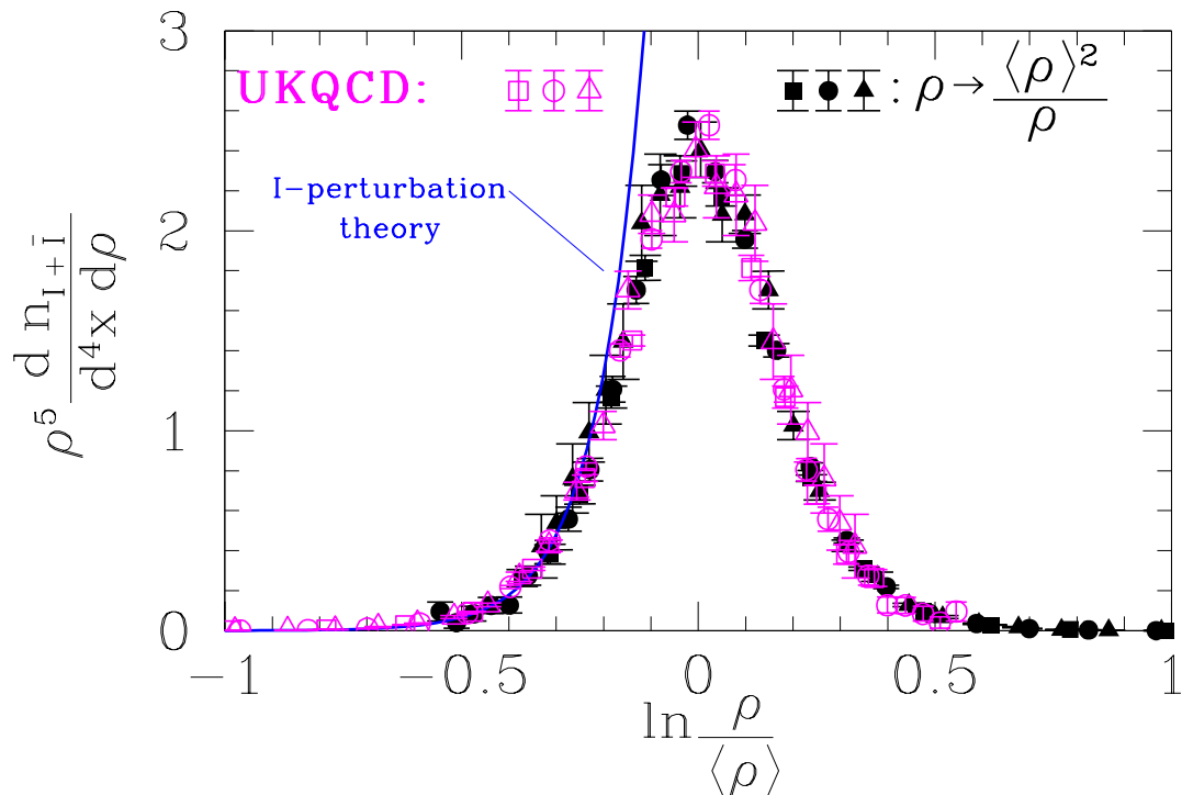
Figure 1: UKQCD lattice data [6, 7] (open symbols) for the instanton size distribution, displayed such as to suggest a virtually perfect inversion symmetry under \rho \rightarrow \langle \rho \rangle^2 / \rho with \langle \rho \rangle \approx 0.6 fm (open and solid data symbols fit onto one universal, symmetric curve). The solid line corresponds to the parameter-free prediction of instanton perturbation theory [7] using the lattice result \Lambda_{\overline{\text{MS}} n_f=0} = (238 \pm 19) MeV from the ALPHA collaboration [9].
