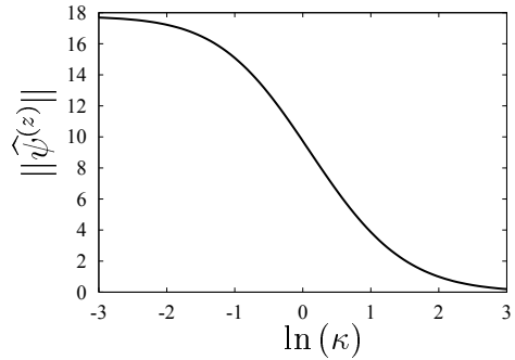
Figure 6: Translation zero modes
