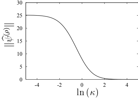
Figure 3: Dilatation zero mode
