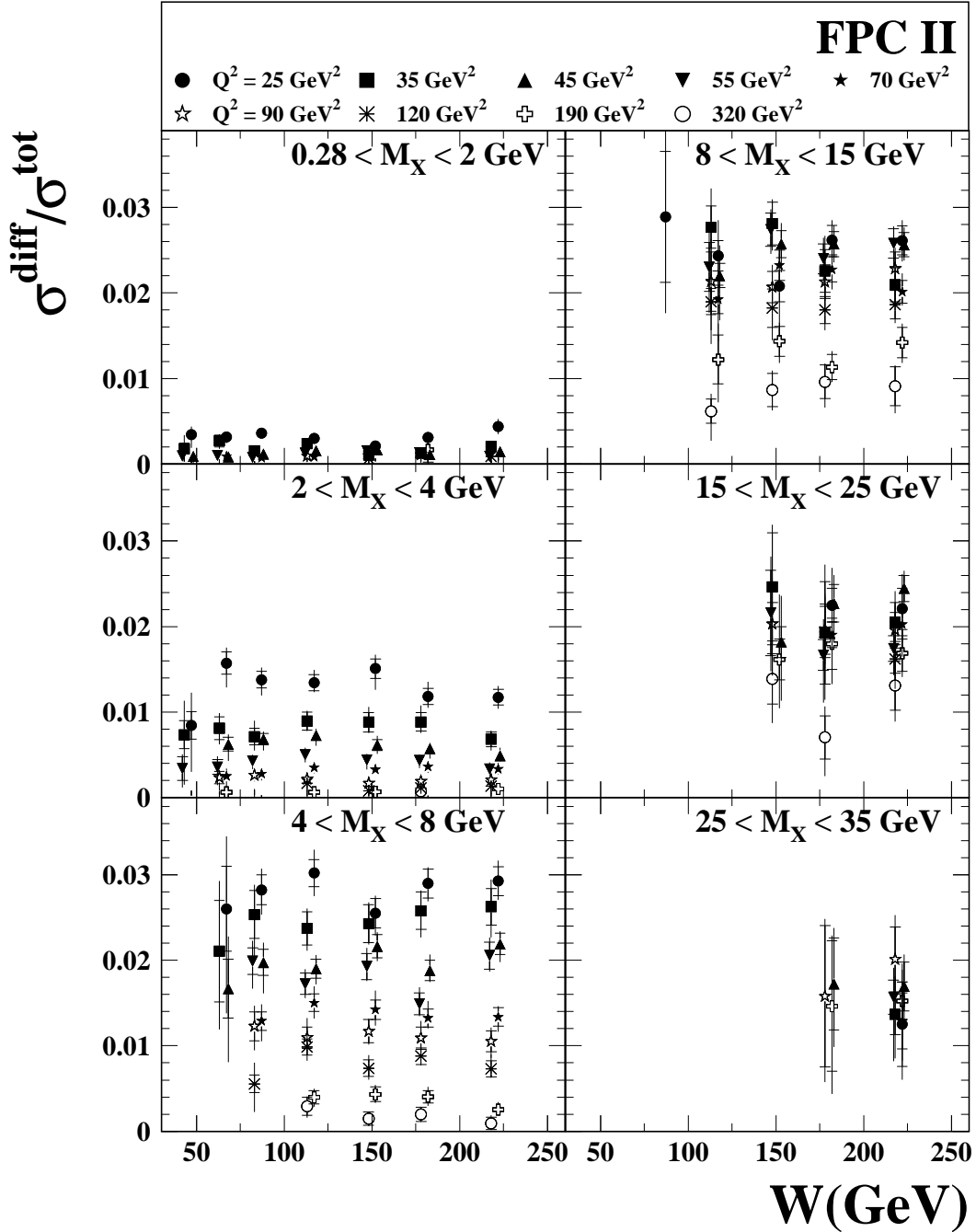
Figure 15: The ratio of the diffractive cross section, integrated over the M_X intervals indicated, \int_{M_a}^{M_b} dM_X d\sigma_{\gamma^*p \rightarrow XN, M_N < 2.3 \text{ GeV}}^{\text{diff}} / dM_X , to the total \gamma^*p cross section, r_{\text{tot}}^{\text{diff}} = \sigma_{\text{diff}}^{\text{diff}} / \sigma_{\gamma^*p}^{\text{tot}} , as a function of W for the Q^2 values indicated, for the FPC II data. The inner error bars show the statistical uncertainties and the full bars the statistical and systematic uncertainties added in quadrature.
