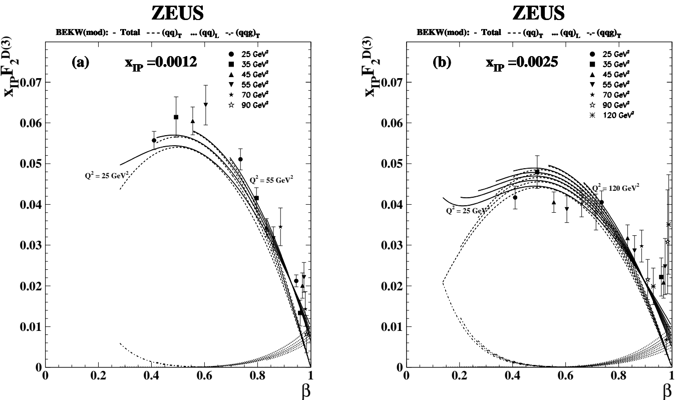
Figure 25: The diffractive structure function of the proton multiplied by x_{\text{IP}} , x_{\text{IP}} F_2^{D(3)} , as a function of \beta for the Q^2 values indicated, at fixed (a) x_{\text{IP}} = 0.0012 and (b) x_{\text{IP}} = 0.0025 , for the FPC I and FPC II data. The curves show the results of the BEKW(mod) fit for the contributions from (qq) for transverse (dashed) and longitudinal photons (dotted) and for the (qgg) contribution for transverse photons (dashed-dotted) together with the sum of all contributions (solid), for the \beta -region studied for diffractive scattering.
