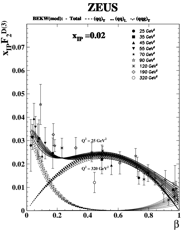
Figure 27: The diffractive structure function of the proton multiplied by x_{\text{IP}} , x_{\text{IP}} F_2^{D(3)} , as a function of \beta for the Q^2 values indicated at fixed x_{\text{IP}} = 0.02 , for the FPC I and FPC II data. The curves show the results of the BEKW(mod) fit for the contributions from (\bar{q}q) for transverse (dashed) and longitudinal photons (dotted) and for the (q\bar{q}g) contribution for transverse photons (dash-dotted) together with the sum of all contributions (solid), for the \beta -region studied for diffractive scattering.
