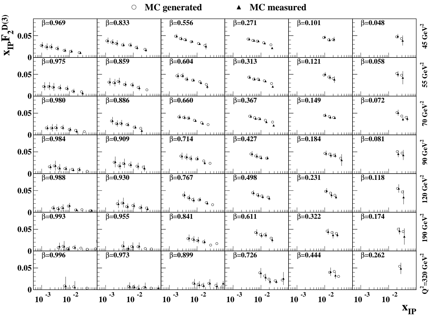
Figure 6: The diffractive structure function of the proton multiplied by x_{\text{IP}} , x_{\text{IP}} F_2^{D(3)} , as a function of x_{\text{IP}} for different regions of \beta and Q^2 : comparison of the MC generated values (open points) with the MC measured values (solid triangles) as determined via the fit to the \ln M_X^2 distributions. The x_{\text{IP}} F_2^{D(3)} values for MC measured are shown at values of x_{\text{IP}} increased by 10%.
