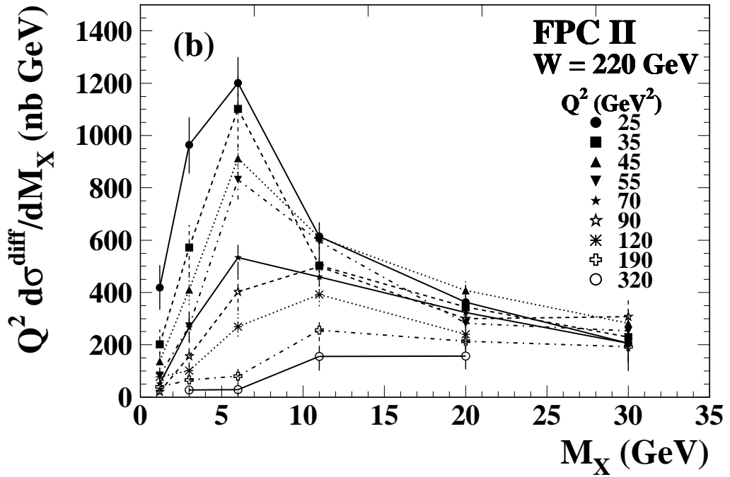
Figure 13: The diffractive cross section multiplied by Q^2 , Q^2 d\sigma_{\gamma^*p \rightarrow XN}^{\text{diff}}/dM_X , M_N < 2.3 GeV, W = 220 GeV as a function of M_X for the Q^2 values indicated, for (a) FPC I data and (b) FPC II data. The inner error bars show the statistical uncertainties and the full bars the statistical and systematic uncertainties added in quadrature.
