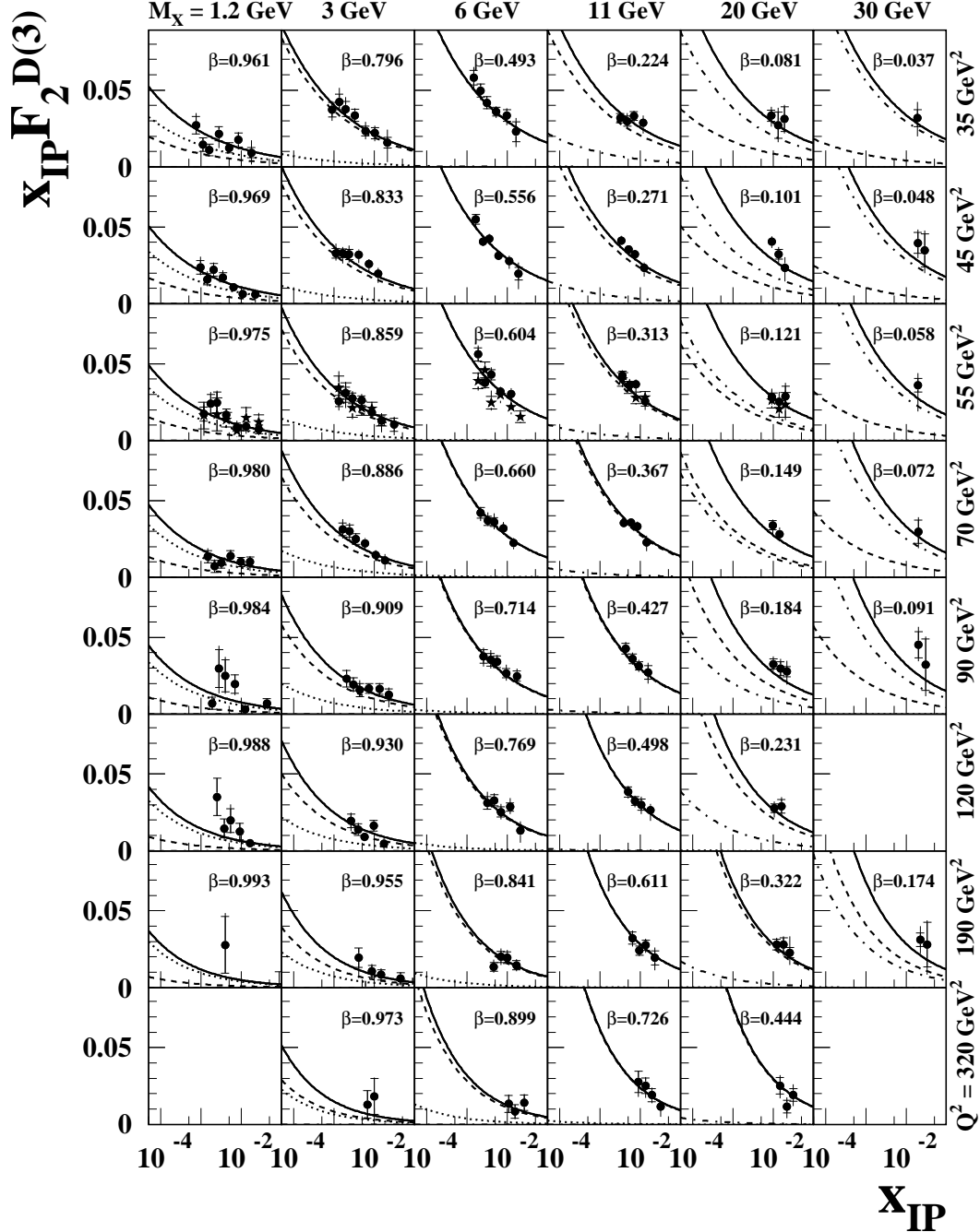
Figure 20: The diffractive structure function of the proton multiplied by x_p , x_p F_2^{D(3)} , for \gamma^* p \rightarrow XN , M_N < 2.3 GeV as a function of x_p for different regions of \beta and Q^2 \geq 35 GeV 2 : both FPC I data (stars) and FPC II data (dots) are shown. The inner error bars show the statistical uncertainties and the full bars the statistical and systematic uncertainties added in quadrature. The curves show the results of the BEKW(mod) fit for the contributions from (q\bar{q}) for transverse (dashed) and longitudinal photons (dotted) and for the (q\bar{q}g) contribution for transverse photons (dashed-dotted) together with the sum of all contributions (solid). For display purposes, some of the x_p F_2^{D(3)} values at Q^2 = 90, 120, 190 and 320 GeV 2 with large uncertainties are not shown but given in Tables 27 – 29.
