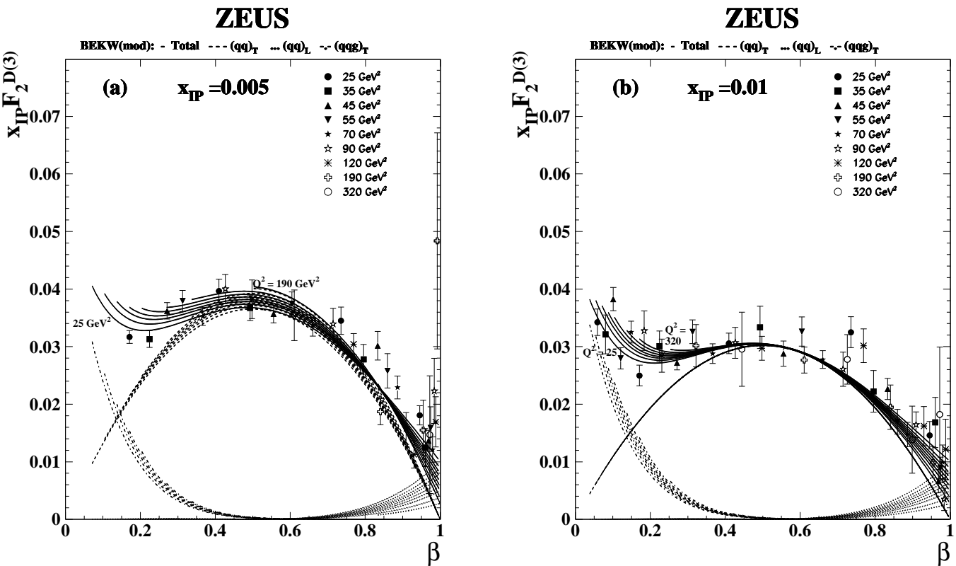
Figure 26: The diffractive structure function of the proton multiplied by x_p , x_p F_2^{D(3)} , as a function of \beta for the Q^2 values indicated, at fixed (a) x_p = 0.005 and (b) x_p = 0.01 , for the FPC I and FPC II data. The curves show the results of the BEKW(mod) fit for the contributions from (q\bar{q}) for transverse photons (dashed) and longitudinal photons (dotted) together with the sum of all contributions (solid), for the \beta -region studied for diffractive scattering.
