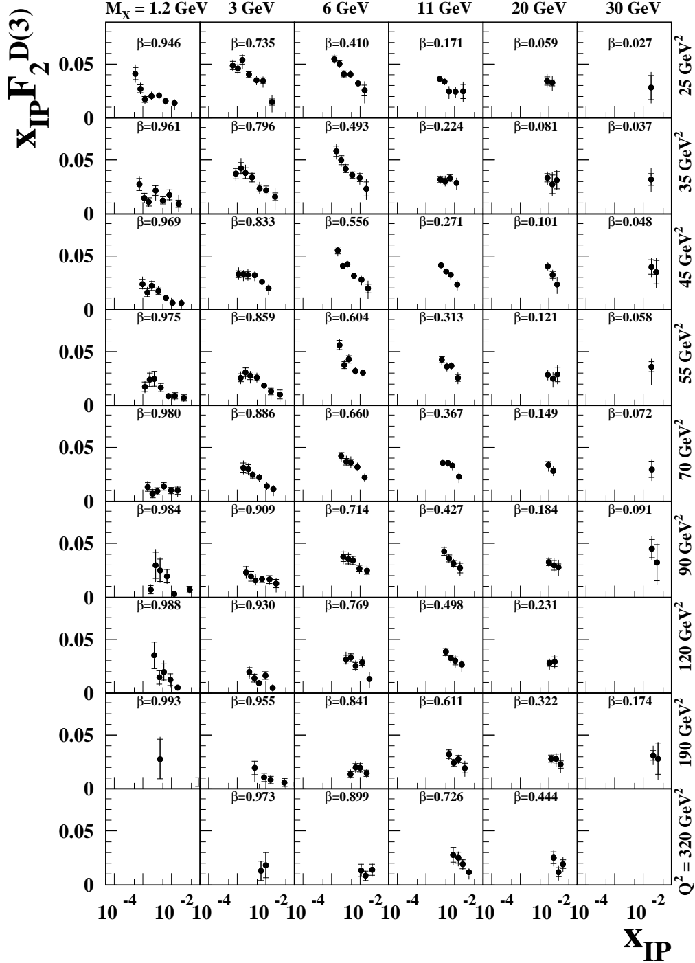
Figure 18: The diffractive structure function of the proton multiplied by x_p , x_p F_2^{D(3)} , for \gamma^* p \rightarrow XN , M_N < 2.3 GeV as a function of x_p for different regions of \beta and Q^2 , for the FPC II data. The inner error bars show the statistical uncertainties and the full bars the statistical and systematic uncertainties added in quadrature. For display purposes, some of the x_p F_2^{D(3)} values at Q^2 = 90, 120, 190 and 320 GeV 2 with large uncertainties are not shown but given in Tables 25 – 29.
