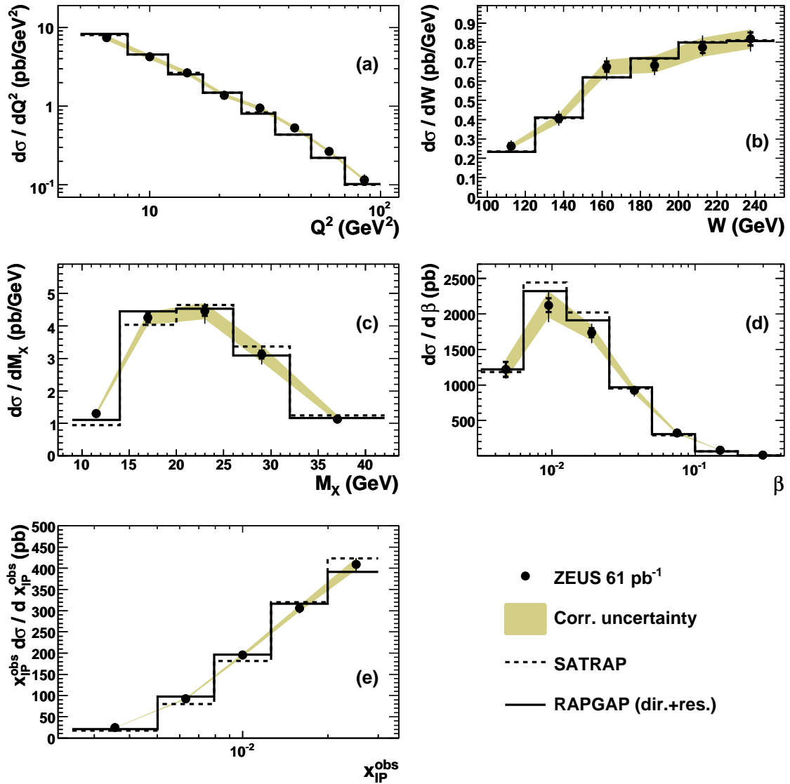
Figure 3: Measured differential cross section (dots) as a function of (a) Q^2 , (b) W , (c) M_X , (d) \beta and (e) x_{IP}^{\text{obs}} . The inner error bars represent the statistical uncertainty and the outer error bars represent the statistical and uncorrelated systematic uncertainties added in quadrature. The shaded band represents the correlated uncertainty. For comparison the area-normalised predictions of the RAGGAP (solid lines) and the SATRAP (dashed lines) MC models are also shown.
