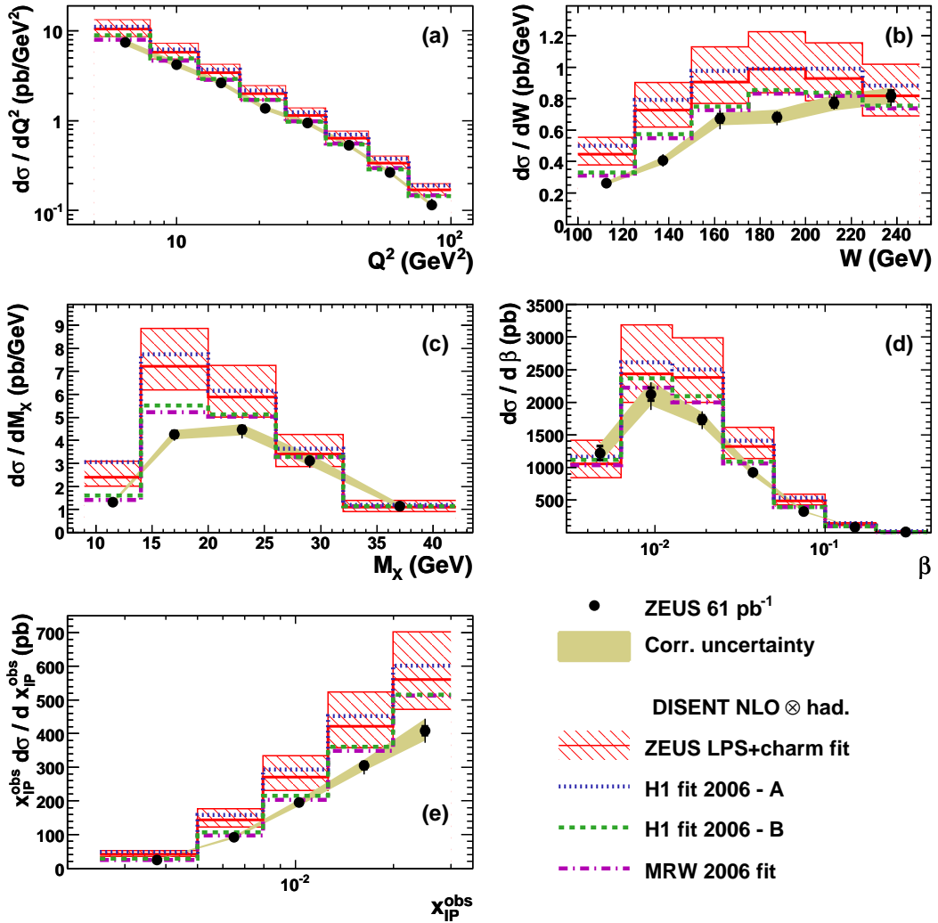
Figure 5: Measured differential cross section as a function of (a) Q^2 , (b) W , (c) M_X , (d) \beta and (e) x_{\text{IP}}^{\text{obs}} compared to the NLO predictions obtained using the available dPDFs, as indicated in the figure. The hatched area indicates the theoretical uncertainty of the predictions estimated using the ZEUS LPS+charm dPDFs. Other details as in the caption of Fig. 3.
