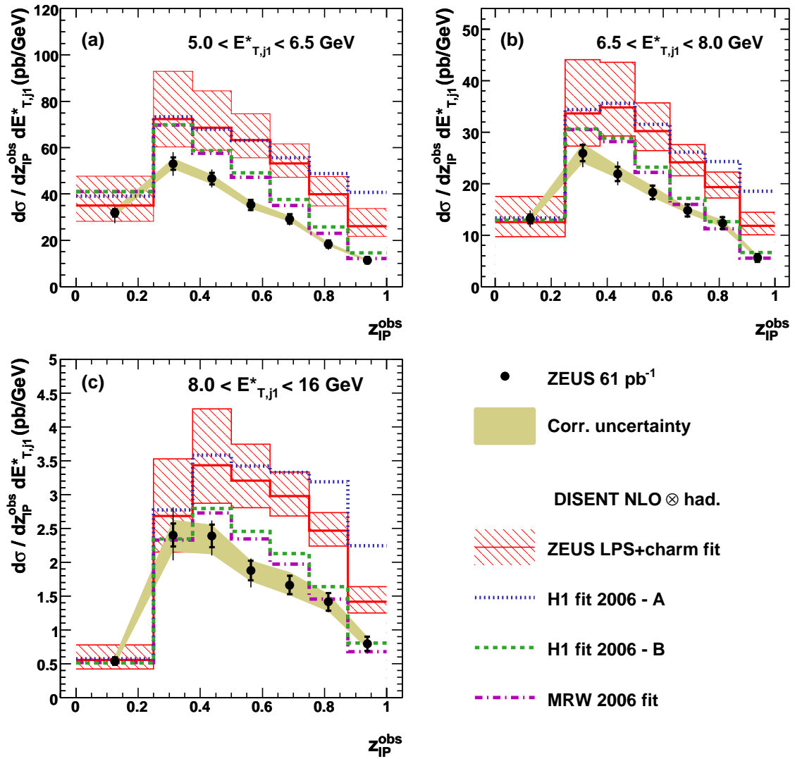
Figure 9: Measured differential cross section as a function of z_{IP}^{obs} in different regions of E_{T,j1}^* (dots). Other details as in the caption of Fig. 5.
