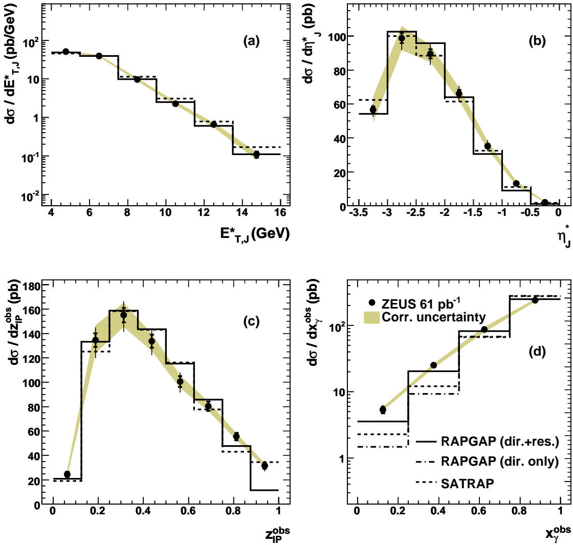
Figure 4: Measured differential cross section as a function of (a) E_{T,J}^* , (b) \eta_J^* , (c) z_{IP}^{obs} and (d) x_\gamma^{obs} . The dashed-dotted line represents the area-normalised RAPGAP with only the direct photon contribution. Other details as in the caption of Fig. 3.
