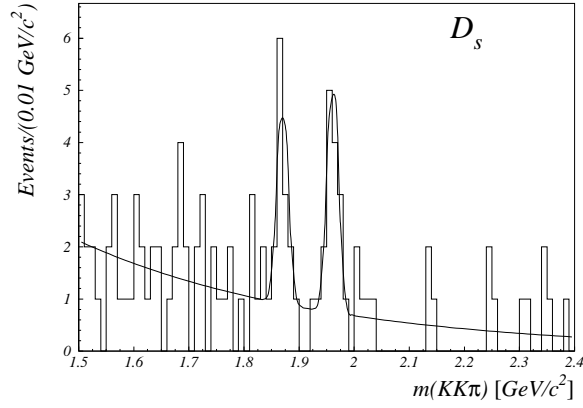
Fig. 3. Invariant mass distributions for \phi\pi^+ \rightarrow (K^- K^+)\pi^+ combinations. Besides the D_s^+ peak at 1.96 \text{ GeV}/c^2 , a D^+ peak at 1.87 \text{ GeV}/c^2 is also visible. This peak corresponds to the Cabibbo suppressed decay D^+ \rightarrow \phi\pi^+ . The curve shows the result of a maximum likelihood fit to the data.
