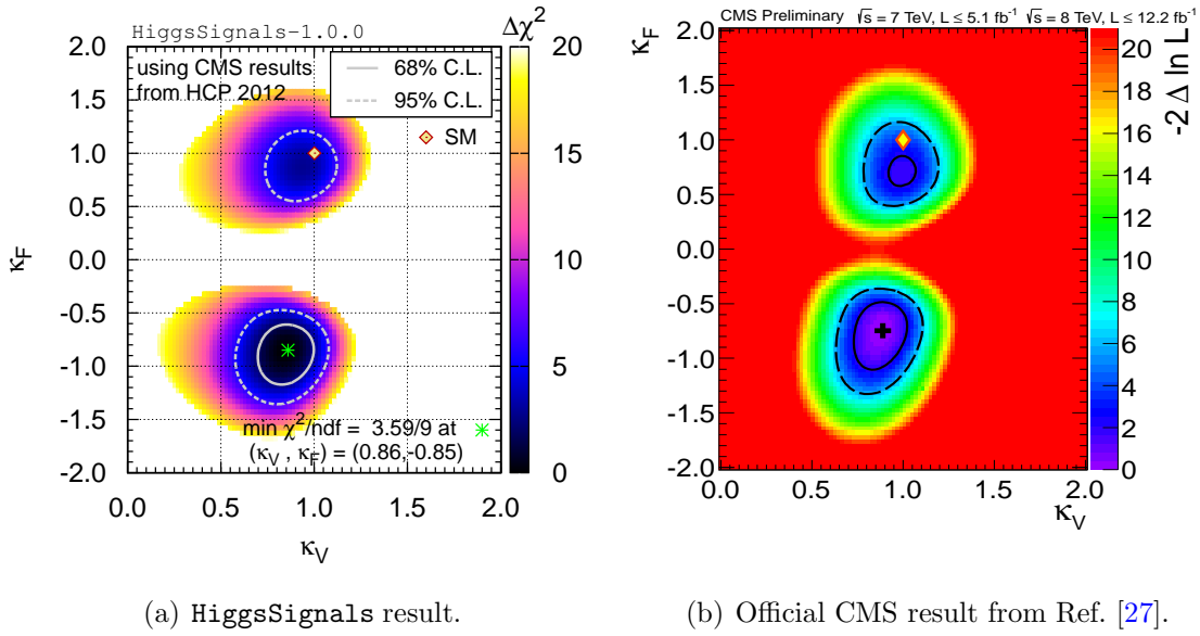
Figure 7. Comparison of the two-parameter fits probing different coupling strength scale factors for fermions, \kappa_F , and vector bosons, \kappa_V , obtained using HiggsSignals (a), and by CMS [27] (b). The signal strength measurements used for the HiggsSignals fit are listed in Tab. 11. The Higgs mass is chosen to be m_H = 125.8 GeV.
