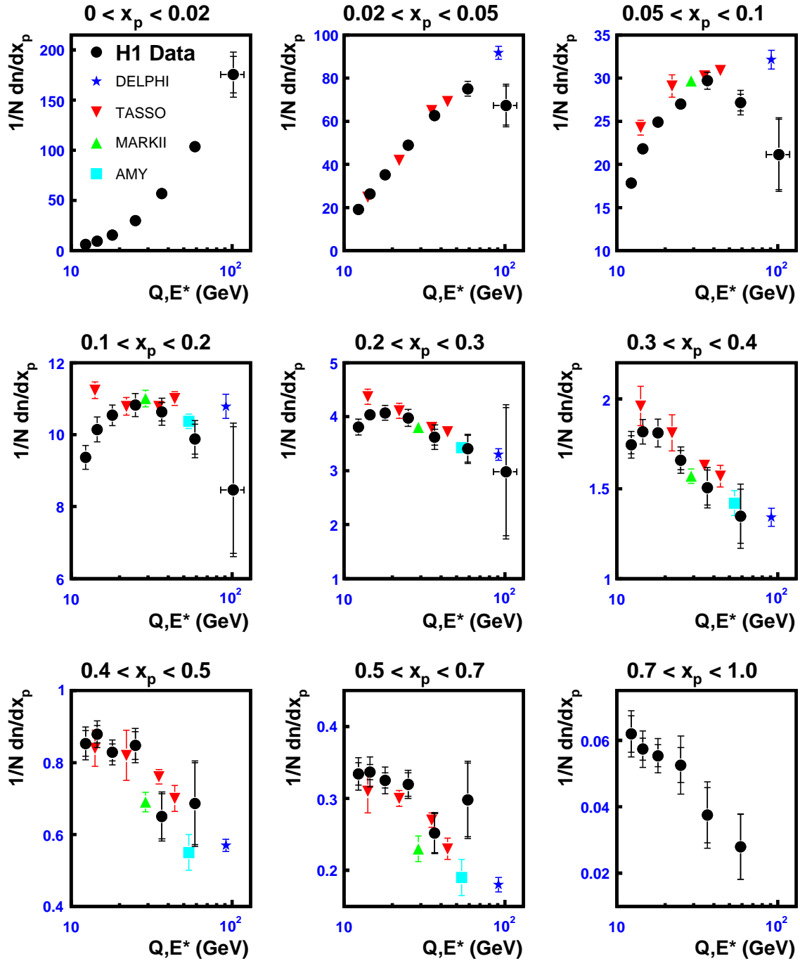
Figure 2: The measured normalised distributions of the scaled momentum, \frac{1}{N} \frac{dn}{dx_p} , as a function of Q for nine different x_p regions. The statistical error is shown by the inner error bar and the outer error bar represents the statistical and systematic error added in quadrature. In addition there is a further correlated error of \sim 0.5 - 7\% (increasing with x_p ) coming from the electron energy scale uncertainty (not shown). The data are displayed at the average value of Q , the horizontal error bars represent the statistical errors given in table 1. Data are compared to results from various e^+e^- experiments (taking Q = E^* ). Note the suppressed zeros and large change in scale of the vertical axis moving to higher values of x_p .
