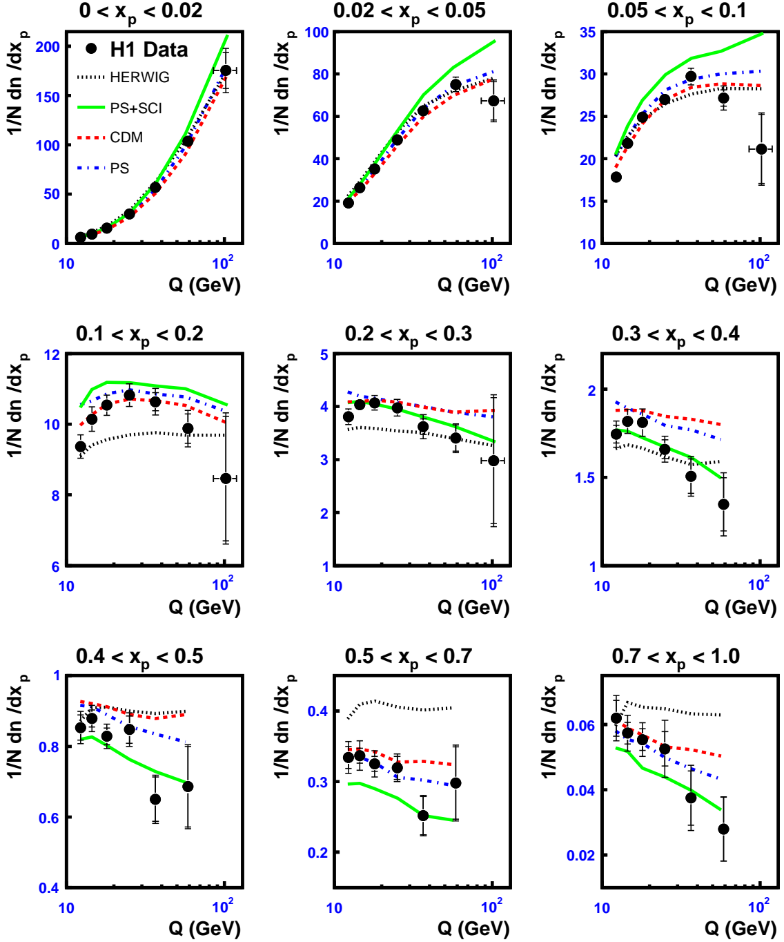
Figure 3: The measured normalised distributions of the scaled momentum, \frac{1}{N}dn/dx_p , as a function of Q for nine different x_p regions. The statistical error is shown by the inner error bar and the outer error bar represents the statistical and systematic error added in quadrature. In addition there is a further correlated error of \sim 0.5 - 7\% (increasing with x_p ) coming from the electron energy scale uncertainty (not shown). The data are displayed at the average value of Q , the horizontal error bars represent the statistical errors given in table 1. The data are compared to predictions from different models of the parton cascade and hadronisation processes implemented in leading order matrix element Monte Carlo programs as described in the text.
