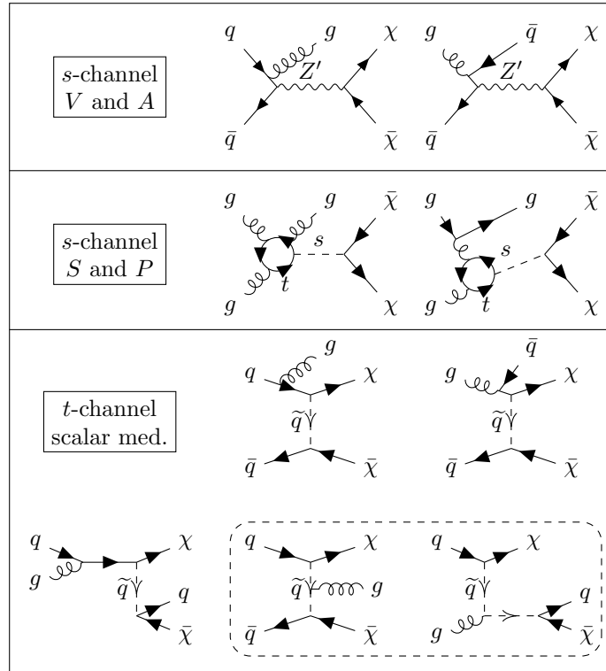
Figure 2: Feynman diagrams for the production of a DM pair in association with a quark or a gluon, leading to a mono-jet signature. Additional diagrams obtained by exchanging a fermion and a anti-fermion, as well as the ones obtained by permuting the gluon vertices in the loop in the (pseudo-)scalar case, are neglected. The diagrams enclosed in the dashed box in the t -channel model are suppressed in the EFT limit.
