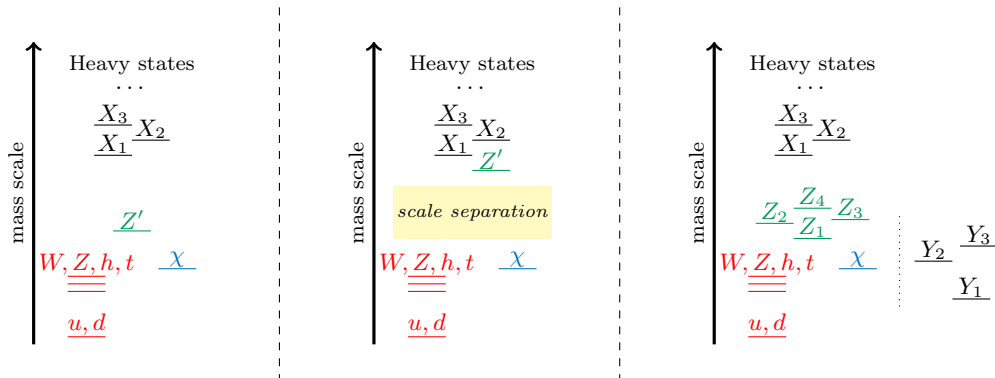
Figure 1: Left: a simplified model viewed as a sector of a more general new physics scenario. The SM is complemented by the DM particle \chi and a mediator Z' . Other heavy states X_1, X_2, X_3, \dots may be integrated out because they are very heavy. Centre: in the case in which the mediator Z' itself has a very large mass, it may be integrated out as well and the interaction is mediated by effective operators. Right: In a generic setup the DM-SM interaction is mediated by a number of operators, possibly interfering with each other. Moreover, additional states Y_1, Y_2, Y_3, \dots that do not couple directly to DM may be present. Those states can constitute a new handle on the dark sector, other than DM. The ‘less simplified’ models described in section 4 fall in this category.
