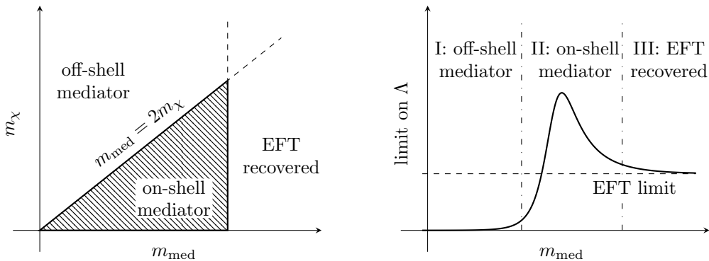
Figure 3: Left: Sketch of the limits obtained from mono- X analysis in the m_{\text{med}} - m_{\chi} plane ( left , adapted from [32]) and in the m_{\text{med}} - \Lambda plane ( right , adapted from [36]).
