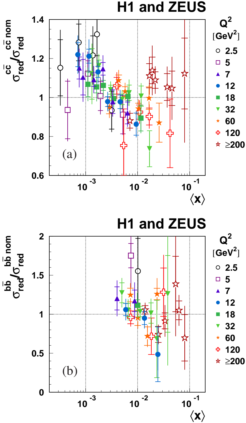
Figure 18: Ratio of the combined reduced cross sections, (a) \sigma_{\text{red}}^{\bar{c}c} and (b) \sigma_{\text{red}}^{\bar{b}b} , to the respective NLO FFNS cross-section predictions, \sigma_{\text{red}}^{\text{nom}} , based on HERAPDF-HQMASS, as a function of the partonic \langle x \rangle for different values of Q^2 .
