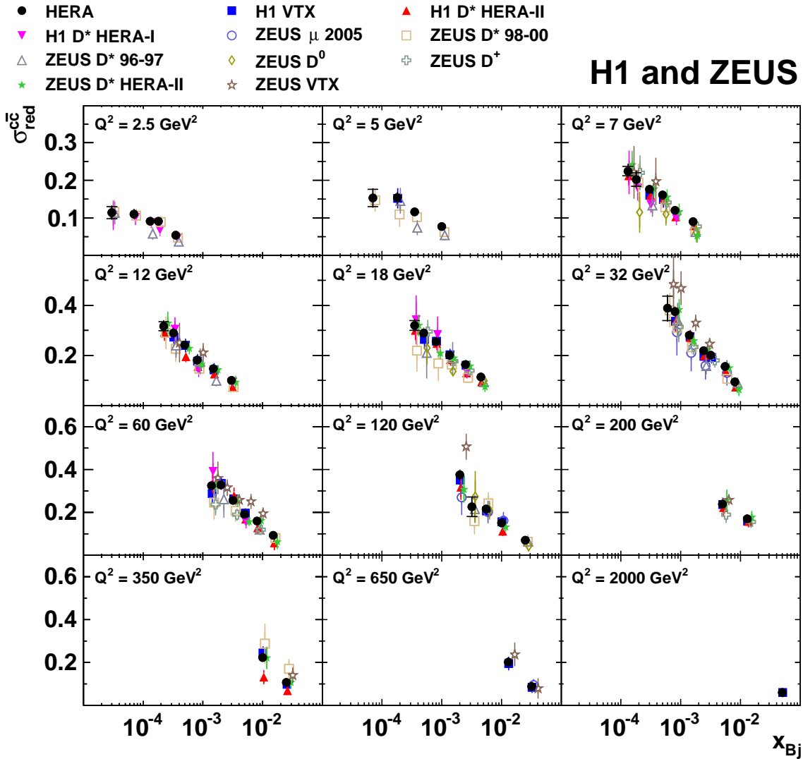
Figure 2: Combined measurements of the reduced c\bar{c} charm production cross sections, \sigma_{\text{red}}^{c\bar{c}} , (full circles) as a function of x_{Bj} for different values of Q^2 . The inner error bars indicate the uncorrelated part of the uncertainties and the outer error bars represent the total uncertainties. The input measurements with their total uncertainties are also shown by different markers. For better visibility the individual input data are slightly displaced in x_{Bj} towards larger values.
