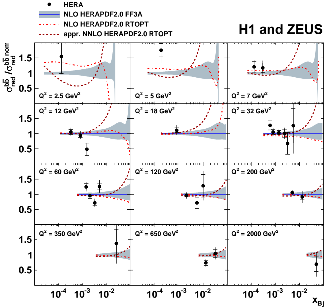
Figure 11: Ratio of reduced beauty cross sections, \sigma_{red}^{b\bar{b}} , as a function of x_{Bj} for given values of Q^2 for the combined data (full circles) and the NLO (dashed-dotted lines) and approximate NNLO (dashed lines) VFNS predictions, obtained using the respective HERAPDF2.0 PDF sets, with respect to the FFNS NLO predictions, \sigma_{red}^{b\bar{b} \text{ nom}} , obtained using HERAPDF2.0 FF3A (solid lines with shaded uncertainty bands). The uncertainties for the VFNS predictions (not shown) are of similar size to those presented for the FFNS calculation.
