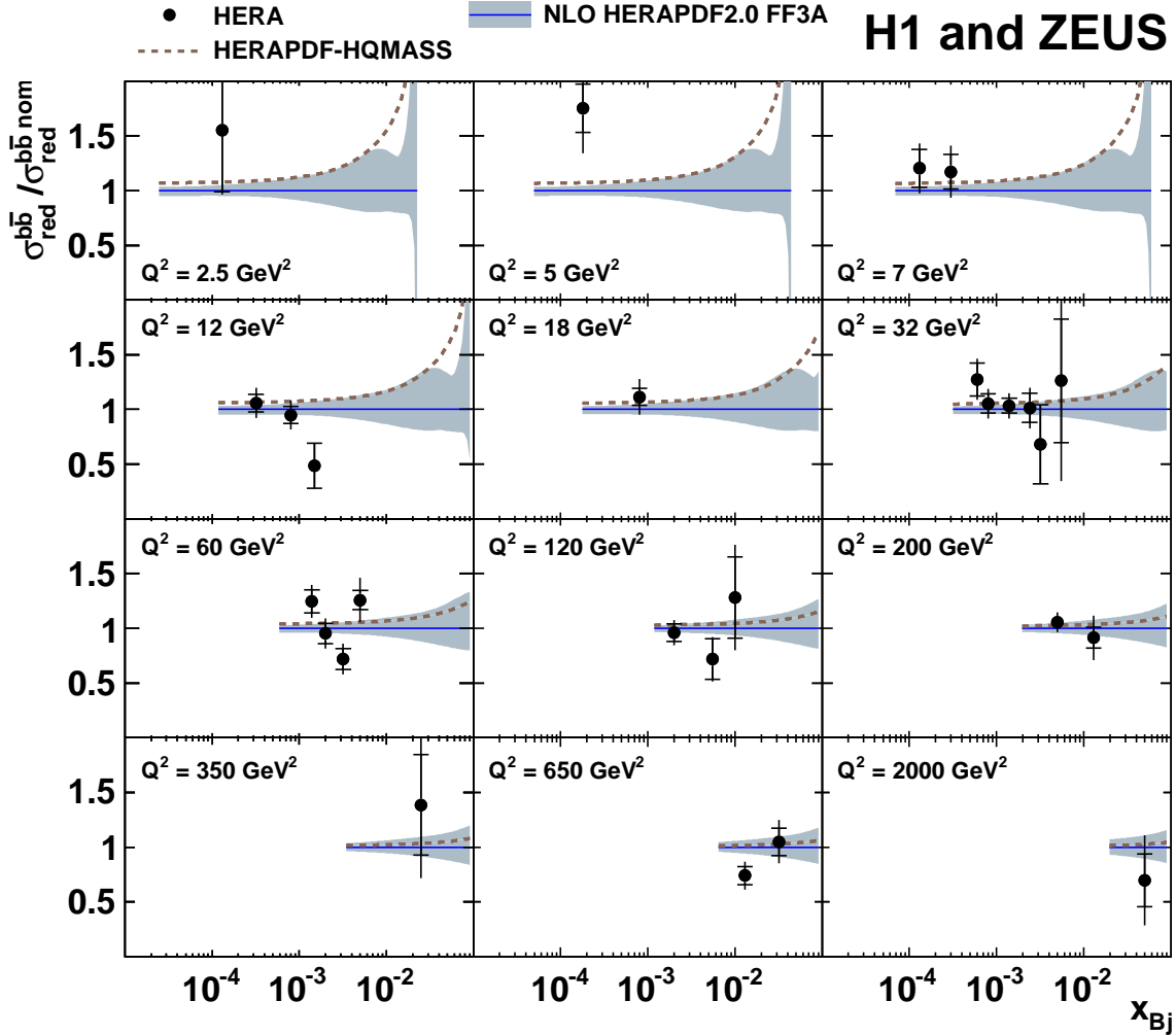
Figure 17: Ratio of reduced beauty cross sections, \sigma_{\text{red}}^{b\bar{b}} , as a function of x_{Bj} for given values of Q^2 for the combined data (full circles) and the NLO FFNS predictions using HERAPDF-HQMASS (dashed lines) with respect to the reference cross sections, \sigma_{\text{red}}^{b\bar{b} \text{ nom}} , based on HERAPDF2.0 FF3A (solid lines with uncertainty bands).
