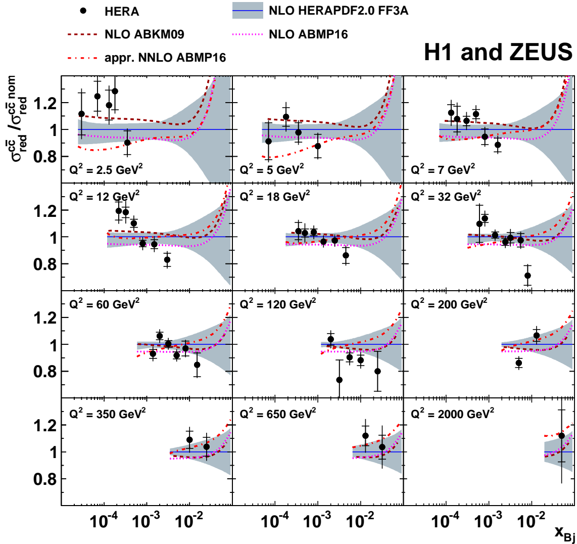
Figure 8: Ratio of reduced charm cross sections, \sigma_{red}^{c\bar{c}} , as a function of x_{Bj} for given values of Q^2 for the combined data (full circles) and the NLO (dashed and dotted lines) and approximate NNLO (dashed-dotted lines) QCD FFNS predictions, obtained using various PDFs, as in figure 6, with respect to the FFNS NLO predictions, \sigma_{red}^{c\bar{c} \text{ nom}} , obtained using HERAPDF2.0 FF3A (solid lines with shaded uncertainty bands).
