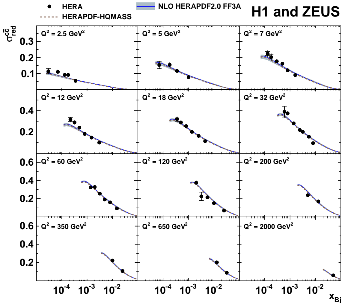
Figure 14: Combined reduced charm cross sections, \sigma_{\text{red}}^{c\bar{c}} , (full circles) as a function of x_{Bj} for given values of Q^2 , compared to the NLO QCD FFNS predictions based on HERAPDF-HQMASS (dashed lines) and on HERAPDF2.0 FF3A (solid lines). The shaded bands on the HERAPDF2.0 FF3A predictions show the theory uncertainties obtained by adding PDF, scale and charm-quark mass uncertainties in quadrature.
