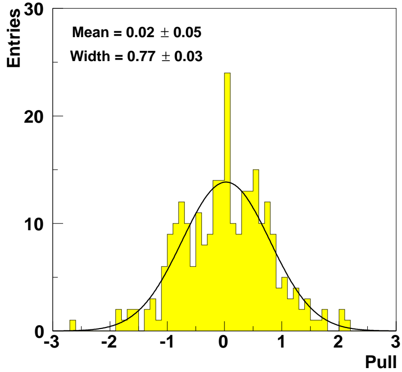
Figure 1: The pull distribution for the combination of the charm and beauty reduced cross sections. The solid line shows a fit of a Gaussian to the pull distribution. The mean and the width quoted are the results from the fit.
