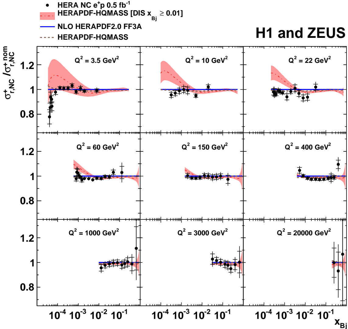
Figure 22: Ratio of combined reduced NC cross sections, \sigma_{r,NC}^+ , (full circles) as a function of x_{Bj} for selected values of Q^2 , compared to the NLO FFNS predictions based on HERAPDF-HQMASS (dashed lines) and those resulting from the alternative fit with x_{Bj} \geq 0.01 required for the inclusive data (dashed-dotted lines), with respect to the reference cross sections, \sigma_{r,NC}^{+,nom} , based on HERAPDF2.0 FF3A (solid lines with uncertainty bands).
