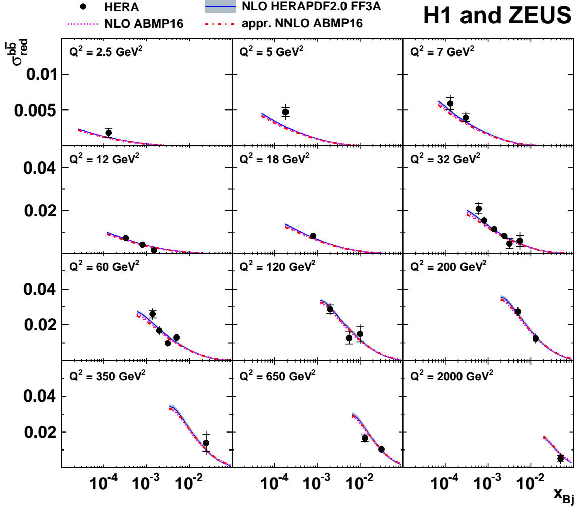
Figure 7: Combined reduced beauty cross sections, \sigma_{red}^{b\bar{b}} , (full circles) as a function of x_{Bj} for given values of Q^2 , compared to the NLO QCD FFNS predictions based on the HERAPDF2.0 FF3A (solid lines) and ABMP16 (dotted lines) PDF sets. Also shown is the approximate NNLO prediction using ABMP16 (dashed-dotted lines). The shaded bands on the HERAPDF2.0 FF3A predictions show the theory uncertainties obtained by adding PDF, scale and beauty-quark mass uncertainties in quadrature.
