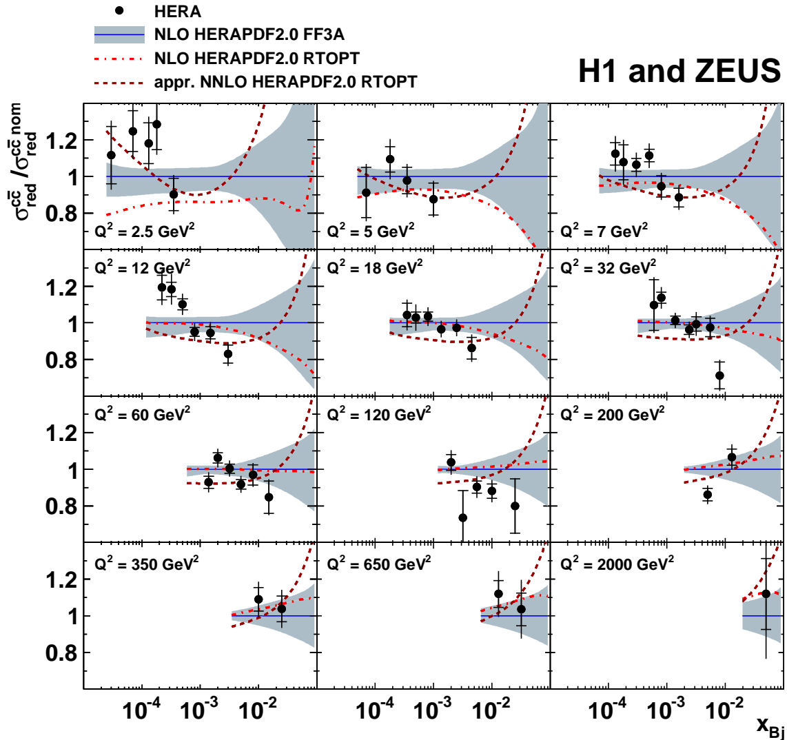
Figure 10: Ratio of reduced charm cross sections, \sigma_{red}^{c\bar{c}} , as a function of x_{Bj} for given values of Q^2 for the combined data (full circles) and the NLO (dashed-dotted lines) and approximate NNLO (dashed lines) VFNS predictions, obtained using the respective HERAPDF2.0 PDF sets, with respect to the FFNS NLO predictions, \sigma_{red}^{c\bar{c} nom} , obtained using HERAPDF2.0 FF3A (solid lines with shaded uncertainty bands). The uncertainties for the VFNS predictions (not shown) are of similar size to those presented for the FFNS calculation.
