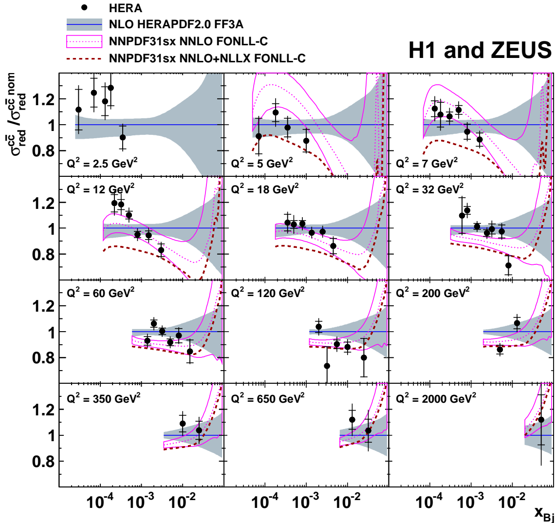
Figure 12: Ratio of reduced charm cross sections, \sigma_{\text{red}}^{c\bar{c}} , as a function of x_{Bj} for given values of Q^2 for the combined data (full circles) and the NNLO VFNS predictions of the NNPDF group with respect to the FFNS predictions, \sigma_{\text{red}}^{c\bar{c}, \text{nom}} , obtained using HERAPDF2.0 FF3A (solid lines with shaded uncertainty bands). Results from two different calculations are shown: without (FONLL-C, dotted lines with uncertainty bands) and with low- x resummation (FONLL-C+NLLsx, dashed lines). For the calculations the NNPDF3.1sx PDF set is used. For better clarity of the presentation the uncertainties of the FONLL+NLLsx calculations are not shown. These are in size similar to those shown for the FONLL calculations. No FONLL predictions based on NNPDF3.1sx are shown at Q^2 = 2.5 \text{ GeV}^2 because this value lies below the starting scale of the QCD evolution in the calculation ( 2.6 \text{ GeV}^2 ).
