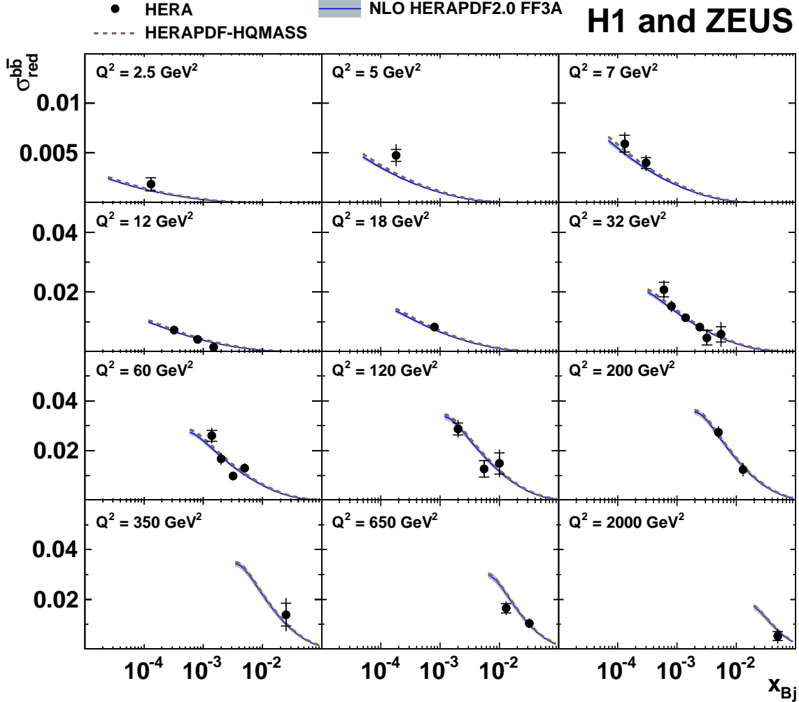
Figure 15: Combined reduced beauty cross sections, \bar{\sigma}_{red}^{bb} , (full circles) as a function of x_{Bj} for given values of Q^2 , compared to the NLO QCD FFNS predictions based on HERAPDF-HQMASS (dashed lines) and on HERAPDF2.0 FF3A (solid lines). The shaded bands on the predictions using the fitted PDF set show the theory uncertainties obtained by adding PDF, scale and beauty-quark mass uncertainties in quadrature.
