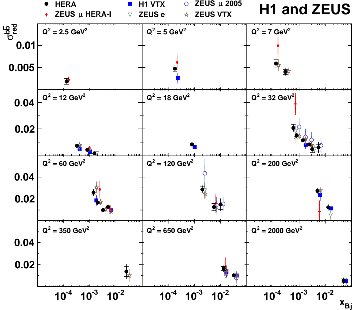
Figure 3: Combined measurements of the reduced b\bar{b} beauty production cross sections, \sigma_{\text{red}}^{b\bar{b}} , (full circles) as a function of x_{Bj} for different values of Q^2 . The inner error bars indicate the uncorrelated part of the uncertainties and the outer error bars represent the total uncertainties. The input measurements with their total uncertainties are also shown by different markers. For better visibility the individual input data are slightly displaced in x_{Bj} towards larger values.
