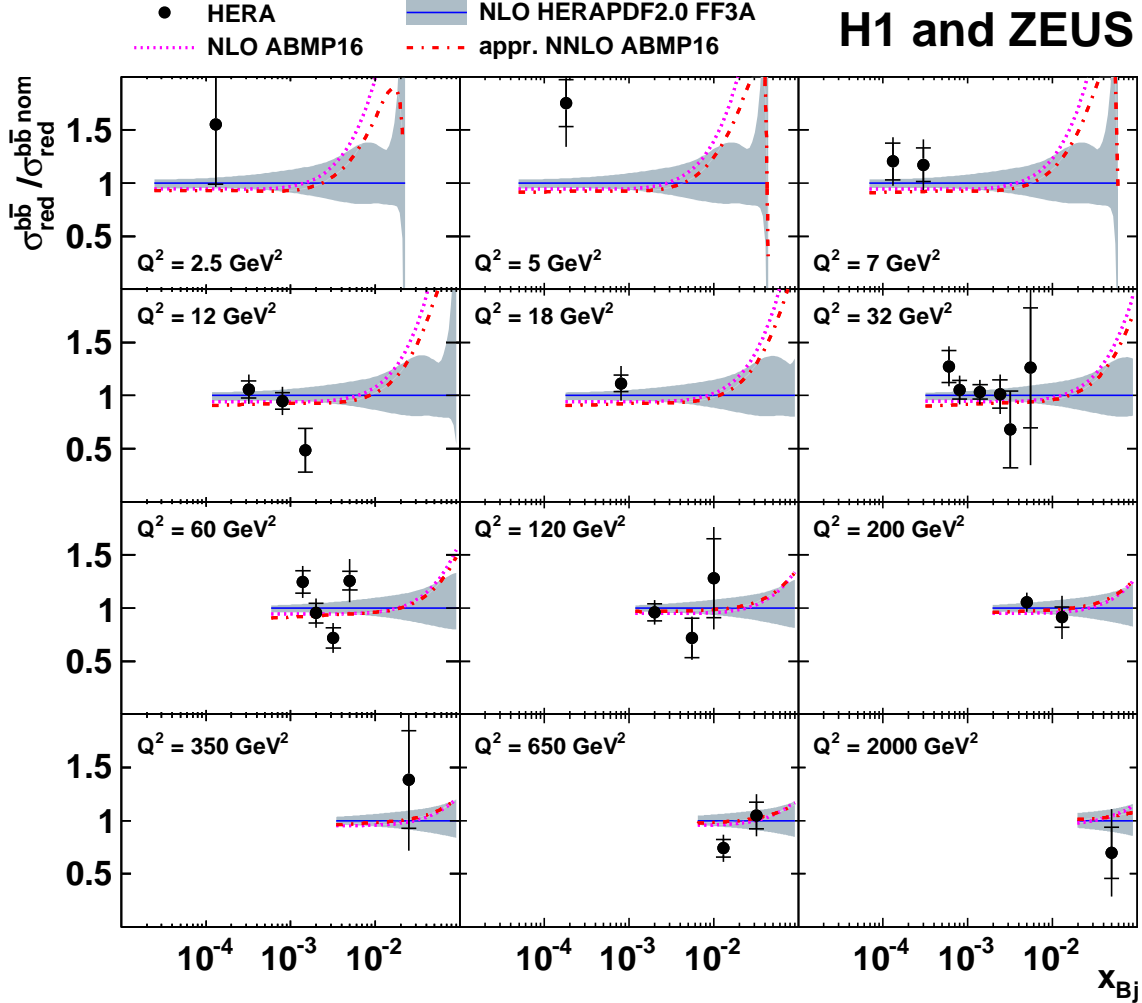
Figure 9: Ratio of reduced beauty cross sections, \sigma_{red}^{b\bar{b}} , as a function of x_{Bj} for given values of Q^2 for the combined data (full circles) and the NLO (dashed and dotted lines) and approximate NNLO (dashed-dotted lines) QCD FFNS predictions, obtained using the same PDF sets as in figure 7, with respect to the FFNS NLO predictions, \sigma_{red}^{b\bar{b} \text{ nom}} , obtained using HERAPDF2.0 FF3A (solid lines with shaded uncertainty bands).
