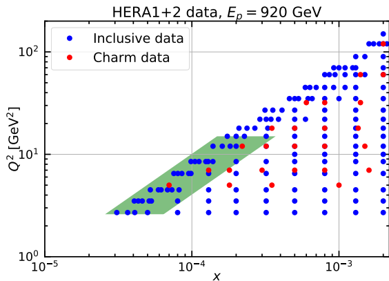
Figure 12 Scatter plot of the low- x and low- Q^2 kinematic region covered by the HERA1+2 inclusive data and charm data at E_p = 920 GeV. The green shaded area indicates the region in which \ln(1/x) resummation has a significant effect as compared to fixed order.
