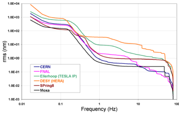
Figure 2: Integrated PSDs of the sites in Fig. 1, at f > 1 Hz cut value, in vertical direction
