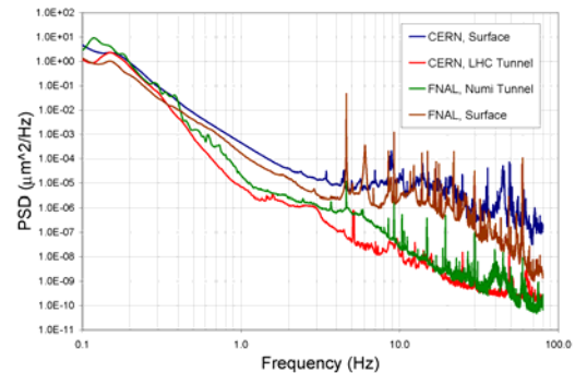
Figure 4: PSD Measurement in the LHC tunnel vs. surface and Numi tunnel in Fermilab vs. surface.
