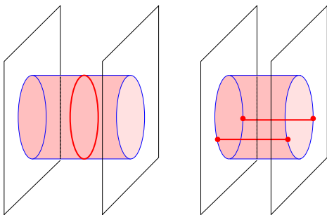
Fig. 4. There are two ways to think about the interaction between two branes. One involves open strings, the other is mediated by closed string modes.
