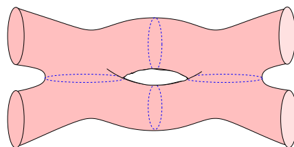
Fig. 1. Any string amplitude can be decomposed into 3-vertices.
