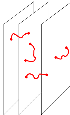
Fig. 3. Open strings can stretch between any pair of branes in a stack. For bookkeeping purposes we introduce the color indices a, b .
