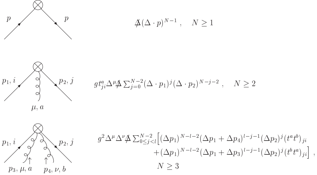
Figure 1: Feynman rules for the operator insertion \otimes to O(a_s^2) , cf. [21]. \Delta denotes a light-like vector, \Delta \cdot \Delta = 0 .
