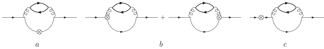
Figure 5: The diagrams contributing to the operator matrix element A_{Qqq}^{\text{NS}} at O(a_s^2) . Weavy lines denote gluons, the full arrow lines are the heavy quark lines, and the thin full lines are light quark lines. The Feynman rules for the operator insertions are given in Figure 1.
