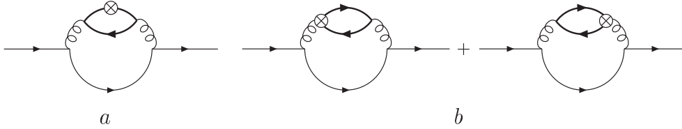
Figure 4: The diagrams contributing to the operator matrix element A_{Qq}^{\text{PS}} at O(a_s^2) . Weavy lines denote gluons, the thick full arrow lines are the heavy quark lines, and the thin full lines are light quark lines. The Feynman rules for the operator insertions are given in Figure 1.
