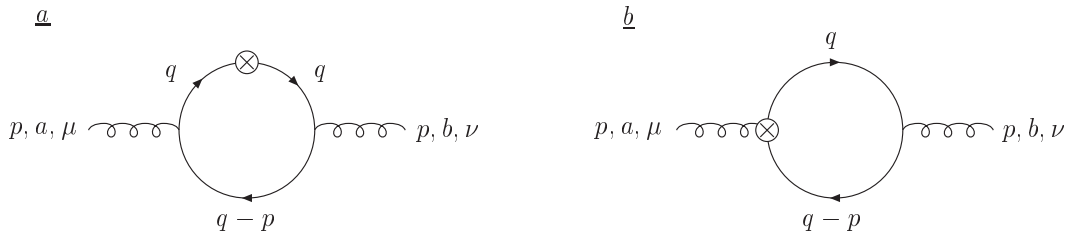
Figure 2: The Feynman diagrams contribution to the operator matrix element A_{Qg} at O(a_s) . Wavy lines denote gluons, and the full arrow lines are the heavy quark lines. The Feynman rules for the operator insertions are given in Figure 1.
