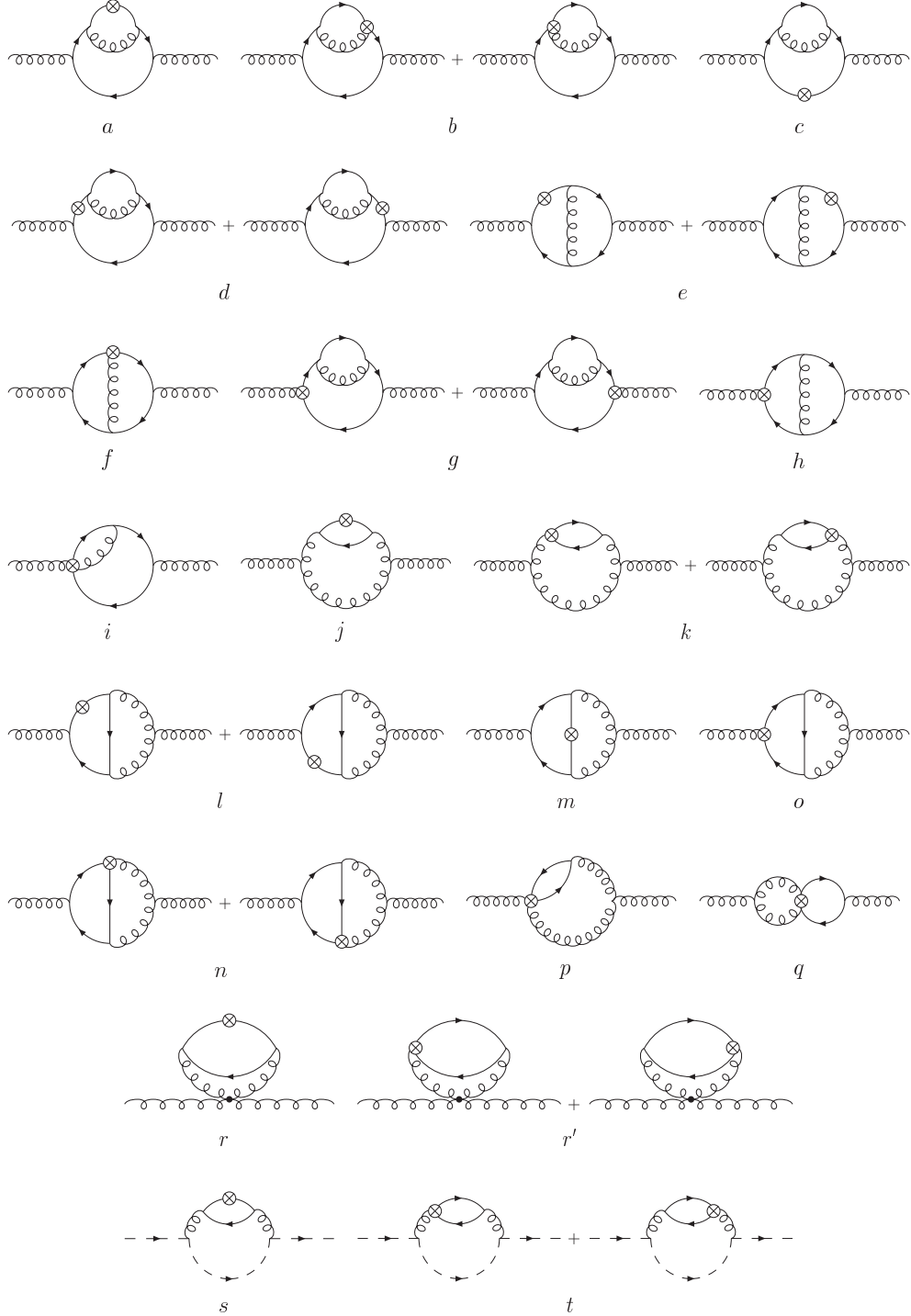
Figure 3: The diagrams contributing to the operator matrix element A_{Qg} at O(a_s^2) . Weavy lines denote gluons, dashed lines ghosts, and the full arrow lines are the heavy quark lines. The Feynman rules for the operator insertions are given in Figure 1.
