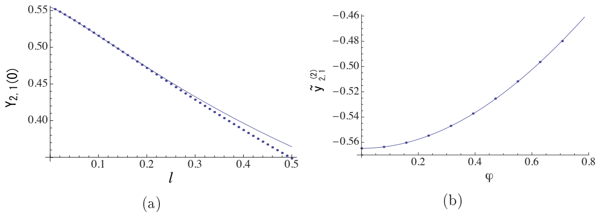
Figure 3: (a) Plots of Y_{2,1}(0) from numerics (points) and from the analytic expansion (solid line) for m_1 = m_2 = l . (b) Phase dependence of an expansion coefficient of \tilde{Y}_{2,1}(0) . The points are from numerical fitting, whereas the solid line represents the analytic expression.
