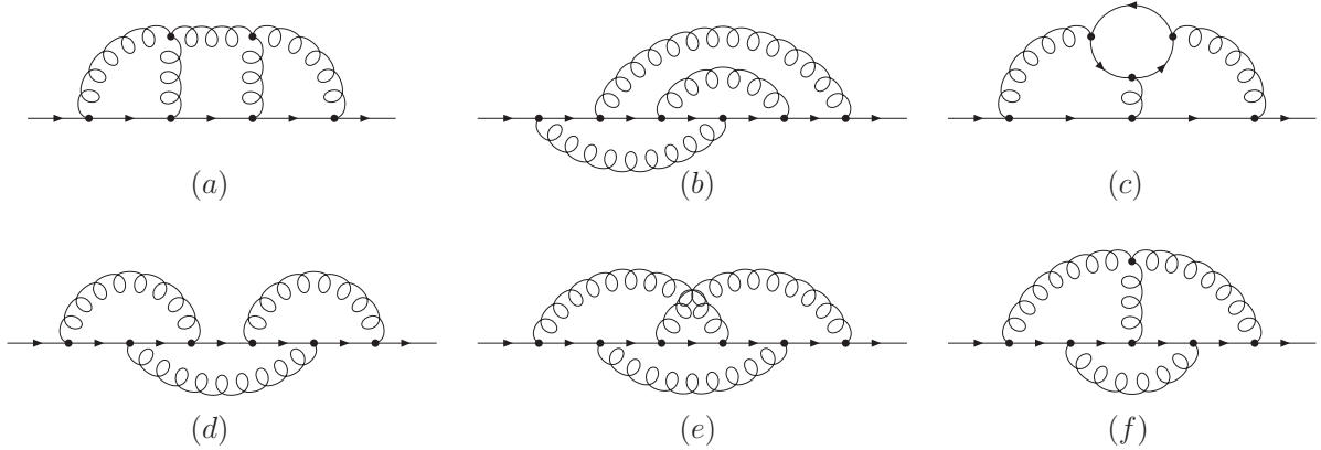
Figure 1: Sample three-loop diagrams. Solid lines denote massive quarks with mass m_q and curly lines denote gluons. In the closed fermion loops all quark flavours have to be considered.
