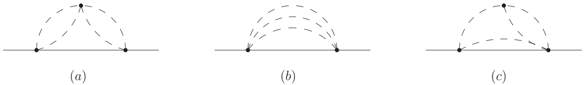
Figure 2: Three-loop master integrals. Solid lines denote massive and dashed lines are massless scalar propagators.
