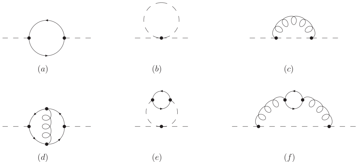
Figure 3: One- and two-loop Feynman diagrams contributing to the \varepsilon -scalar propagator. Dashed lines denote \varepsilon scalars, curly lines denote gluons and solid lines denote massive quarks with mass m_q .
