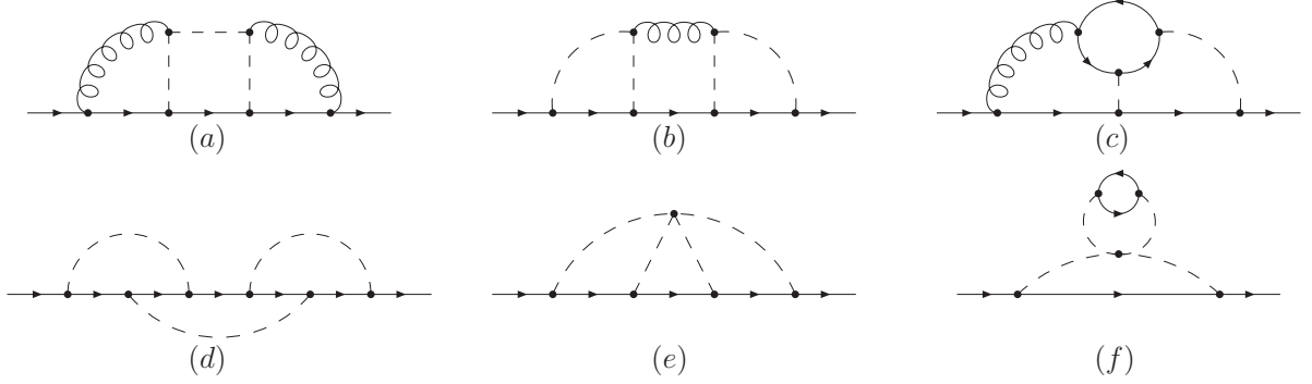
Figure 4: Sample three-loop diagrams contributing to the quark propagator which have to be considered additionally in case dimensional reduction is used for the regularization. Solid lines denote massive quarks with mass m_q , curly lines denote gluons and the \varepsilon scalars are represented by dashed lines. In the closed fermion loops all quark flavours have to be considered.
