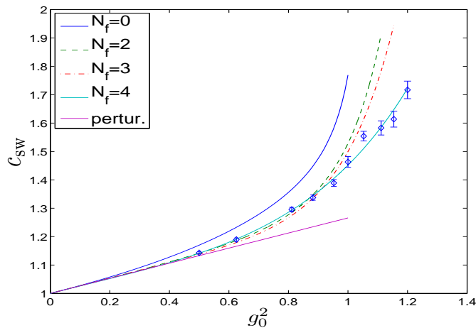
Figure 4: Summary plot of all known c_{\text{sw}}(g_0^2, N_f) for the plaquette gauge action.
