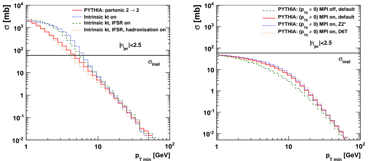
Figure 2: (Left) Cross section from purely partonic 2 \rightarrow 2 process, including intrinsic k_t -effects, including initial and final state parton showers (IFSR) and finally hadronisation. (Right) predicted cross section applying p_{T0} \neq 0 and MPI with different underlying event tunes of PYTHIA.
