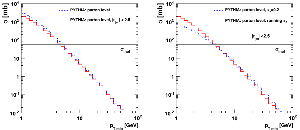
Figure 1: Integrated cross sections at \sqrt{s} = 8 TeV as a function of the minimum transverse momentum: (left) inclusive cross section compared to what can be investigated within |\eta| < 2.5 ; (right) visible inclusive cross section in |\eta| < 2.5 compared to the prediction with fixed \alpha_s = 0.2 .
