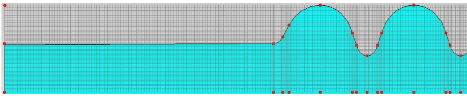
Figure 4.2: A typical mesh used for selected cells in the third harmonic cavity.
