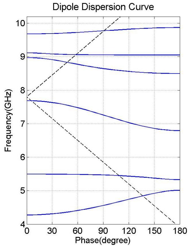
(b) Dipole
