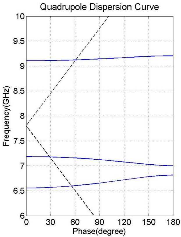
(c) Quadrupole
