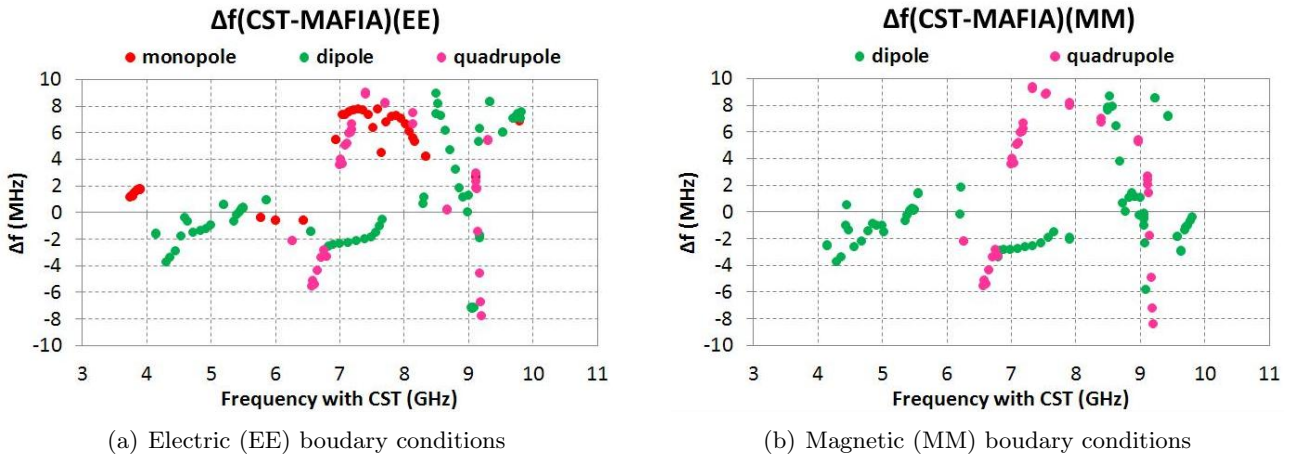
Figure 4.19: Frequency differences of modes simulated with CST® and MAFIA®. \Delta f is calculated as \Delta f = f_{CST} - f_{MAFIA} .
