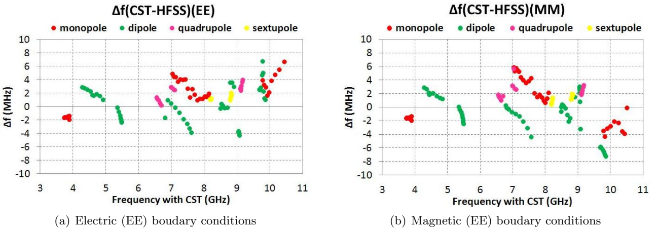
Figure 4.20: Frequency differences of modes simulated with CST® and HFSS®. \Delta f is calculated as \Delta f = f_{CST} - f_{HFSS} .
