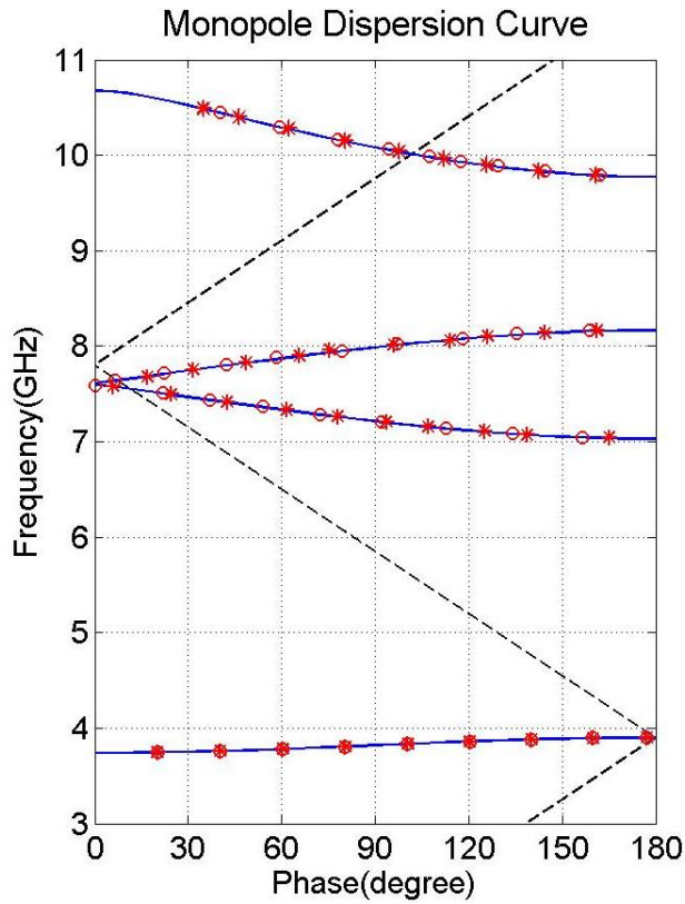
(a) Monopole
