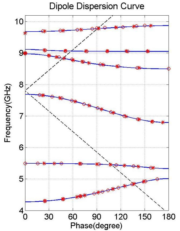
(b) Dipole
