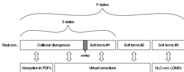
FIG. 2: Overview of the IR singularity structure.
