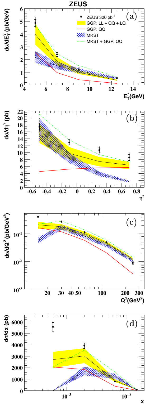
Figure 4: Data points as Fig. 3. Theoretical predictions from Gehrman-De Ridder et al. and Martin et al. are shown with their associated uncertainties indicated by the shaded band and the hatched bands respectively. The dash-dotted line illustrates the combination MRST plus GGP: QQ.
