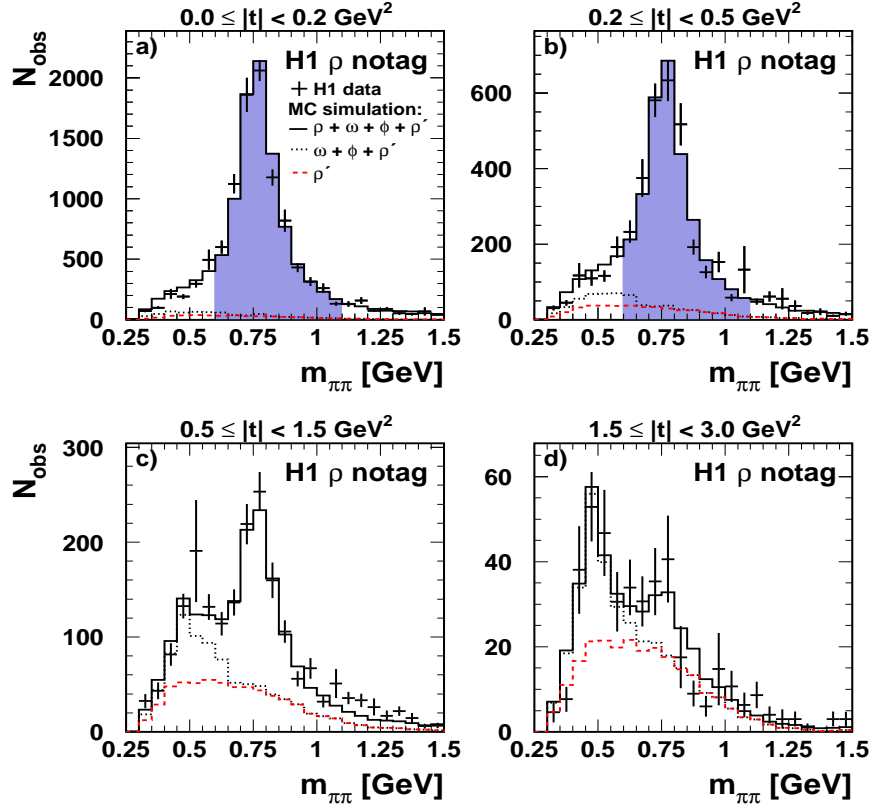
Figure 4: Distributions of the invariant mass m_{\pi\pi} (with the cut m_{KK} > 1.04 \text{ GeV} to reject the \phi \rightarrow KK signal) in four domains in |t| , for the notag sample. The dashed histograms show the MC predictions for the \rho' background, the dotted histograms the sum of the \rho' , \omega and \phi backgrounds, and the full histograms the \rho signal (including interference with \pi\pi non-resonant production) and the sum of all backgrounds. The mass and |t| domain where the cross section measurements are performed is shaded.
