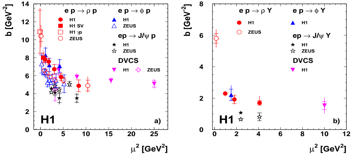
Figure 22: Evolution with the scale \mu^2 = (Q^2 + M_V^2)/4 of the slope parameters b of the exponentially falling |t| distributions of \rho and \phi electroproduction: (a) elastic scattering; (b) proton dissociation. H1 data for DVCS [9], \rho photoproduction [10] and J/\psi production [12, 14] and ZEUS data for \rho [17, 19], \phi [23, 24] and J/\psi [25, 26] production are also presented. For DVCS, the scale is taken as \mu^2 = Q^2 . The present measurements are given in Table 30.
