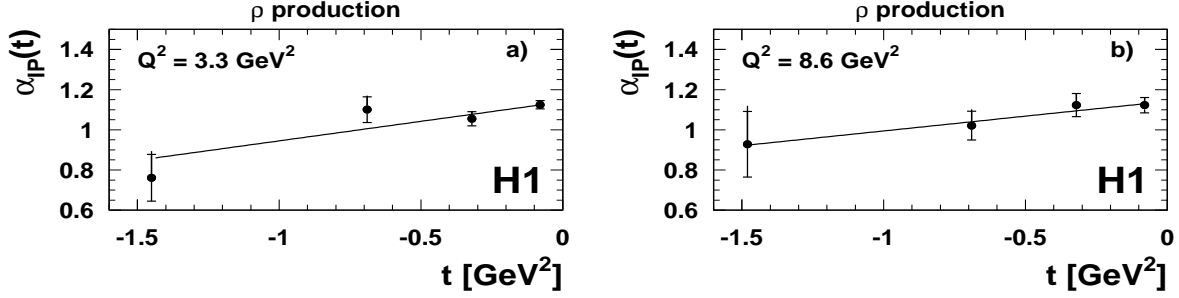
Figure 25: t dependence of the values of the \alpha_P(t) = \delta(t)/4 + 1 parameters obtained from the linear fits to the W dependences shown in Fig. 24 ( \rho production), for (a) Q^2 = 3.3 \text{ GeV}^2 ; (b) Q^2 = 8.6 \text{ GeV}^2 . The lines are the results of linear fits of the form of Eq. (18). The measurements are given in Table 33.
