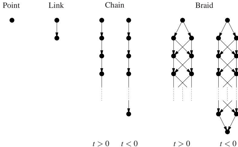
FIGURE 1. The singular vector structure, marked by black circles, of Virasoro Verma modules. Arrows from one vector to another indicate that the latter is a descendant of the former and not vice-versa. Point and link-type Verma modules occur for all central charges. Chain and braid-type modules occur only when t is rational and non-zero. Note that t > 0 corresponds to c \leq 1 and t < 0 corresponds to c \geq 25 .
