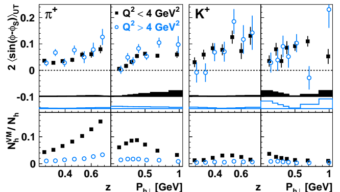
FIG. 2: Sivers amplitudes for \pi^+ (left) and K^+ (right) as functions of z or P_{h\perp} , compared for two different ranges in Q^2 (high- Q^2 points are slightly shifted horizontally). The corresponding fraction of pions and kaons stemming from exclusive vector mesons, extracted from a Monte Carlo simulation, is provided in the bottom panels.
