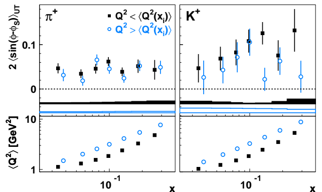
FIG. 3: Sivers amplitudes for \pi^+ (left) and K^+ (right) as functions of x . The Q^2 range for each bin was divided into the two regions above and below \langle Q^2(x_i) \rangle of that bin. In the bottom the average Q^2 values are given for the two Q^2 ranges.
