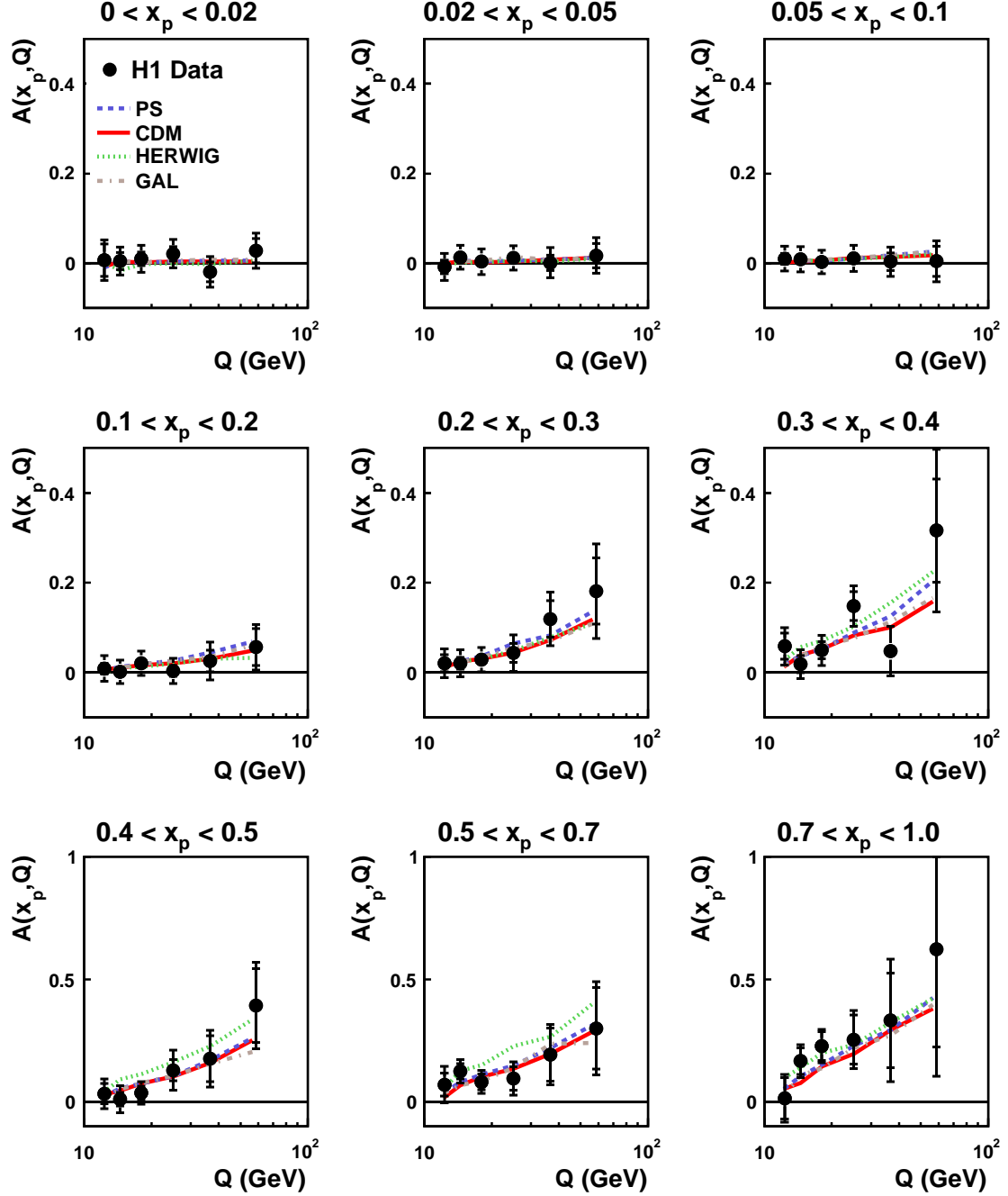
Figure 3: The charge asymmetry, A(x_p, Q) , as a function of Q for nine different x_p regions. The error bars include statistical (inner), and statistical plus systematic errors added in quadrature (outer). The data are displayed at the average value of Q . The data are compared to predictions from different models of the parton cascade and hadronisation processes implemented in leading order matrix element Monte Carlo programs.
