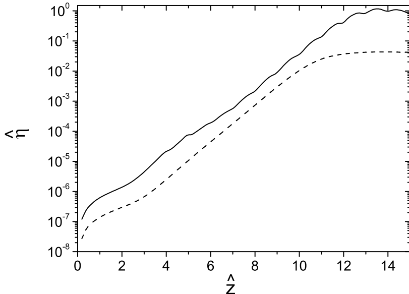
Fig. D.1. Normalized power of the fundamental harmonic (solid) and of the third harmonic (dash) versus normalized undulator length for a SASE FEL. Phase shifts are equal to 2\pi/3 at the positions \hat{z} = 4, 5, 6, \dots, 14 , as suggested in [18]. The undulator parameter is large, K \gg 1 . Definitions of the normalized parameters can be found in [39]
