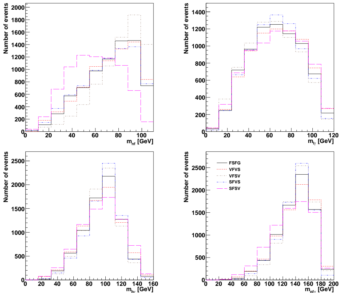
Figure 8: Reconstructed invariant mass distribution from ATLEFAST detector simulation, corresponding to G1a masses and cross sections for 30 \text{ fb}^{-1} integrated luminosity. The histograms have been divided into 10 bins.
