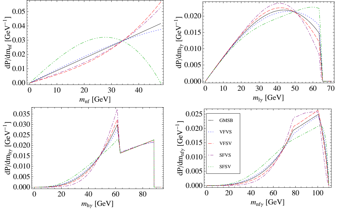
Figure 4: Observable invariant mass distributions for the decay chain in eq. (2.5) for different models and masses from the U1 scenario.
