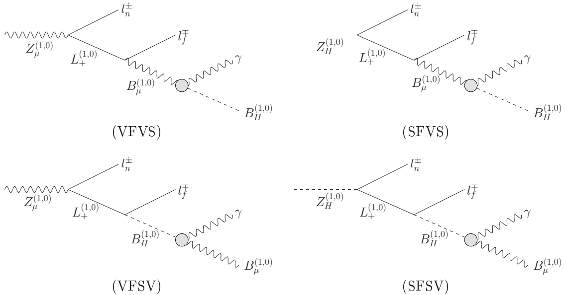
Figure 2: Different UED6 decay chains with various spin configurations leading to the same l^+l^-\gamma + \cancel{E}_\tau signature.
