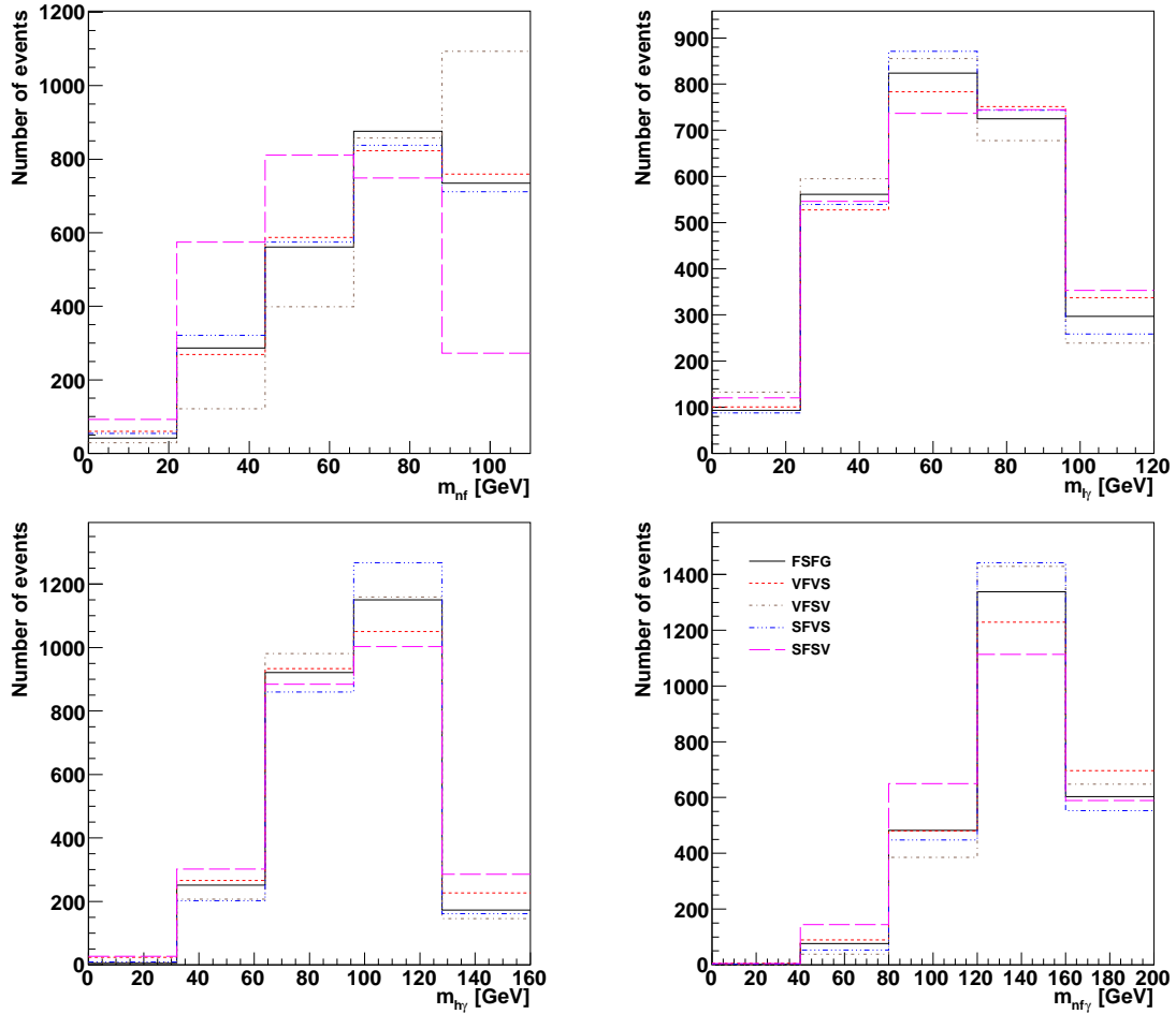
Figure 6: Reconstructed invariant mass distribution from ATLEFAST detector simulation, corresponding to G1a masses and cross sections for 10 \text{ fb}^{-1} integrated luminosity. The histograms have been divided into 5 bins.
