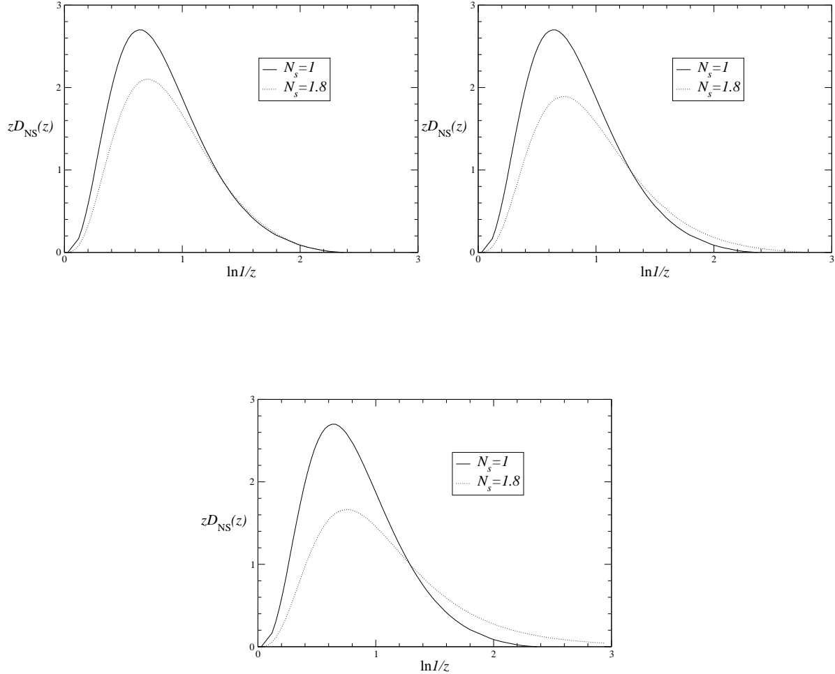
Figure 4: As in Figs. 1 (top left), 2 (top right) and 3 (bottom), but for the non-singlet quark FF with N = 500 , c = 0 , \alpha = 3 and \beta = 3 .
