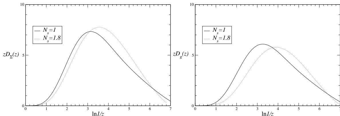
Figure 2: As in Fig. 1, but with f_{ab} = [f_{ab}]_{N_s=1} .
