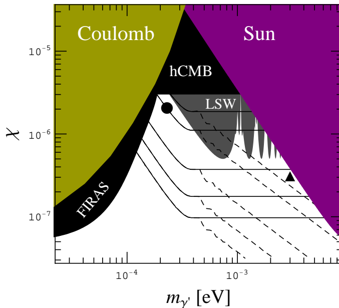
Figure 1: Isocontours of channel capacity (bit/s) for our hidden photon communication system across the Earth’s diameter. From bottom to top the channel capacities are 1, 10, 100, 500, 1000 bit/s. The dashed (solid) lines correspond to setups with (without) phase shift plates. Further details are given in the main text. The dot and triangle are our benchmark points (m_{\gamma'}^{\bullet}, \chi^{\bullet}) and (m_{\gamma'}^{\blacktriangle}, \chi^{\blacktriangle}) . Also shown are current experimental limits on the possible existence of a hidden photon of mass m_{\gamma'} , mixing kinetically with the photon, with a mixing parameter \chi . Strong constraints arise from the non-observation of deviations from the Coulomb law (yellow) [6, 7], from Cosmic Microwave Background (CMB) measurements of the effective number of neutrinos and the blackbody nature of the spectrum (black) [8], from light-shining-through-walls (LSW) experiments (grey) [9–17], and from searches of solar hidden photons with the CAST experiment (purple) [18,19]. The white region in parameter space is currently unexplored, but may be accessed by experiments in the very near future, in particular by improvements in LSW experiments (for proposed experiments probing this region, see Refs. [20–22]).
