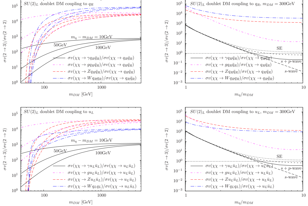
Figure 5: Ratio of three-body and two-body annihilation cross-sections. The top and bottom rows show the case of SU(2)_L doublet dark matter coupling to right-handed up and down-quarks with equal strength ( f = f' ), and to the left-handed up quark, respectively. The left column shows the dependence on the dark matter mass for fixed mass splitting m_\eta - m_{DM} = 10, 50 and 100\text{GeV} , while the right column shows the dependence on the mass of the mediating scalar particle \eta for m_{DM} = 300\text{GeV} . For the relative dark matter velocity we use v = 10^{-3}c .
