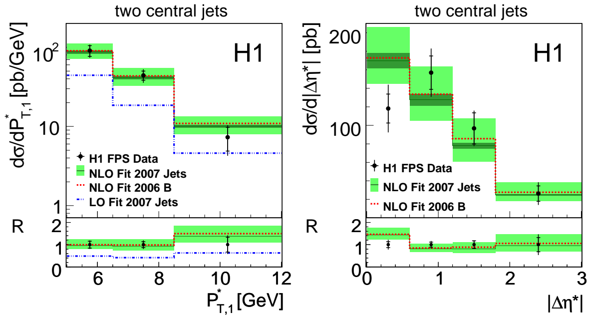
Figure 6: The differential cross section for production of two central jets shown as a function of P_{T,1}^* and |\Delta\eta^*| . For more details see figure 5.
