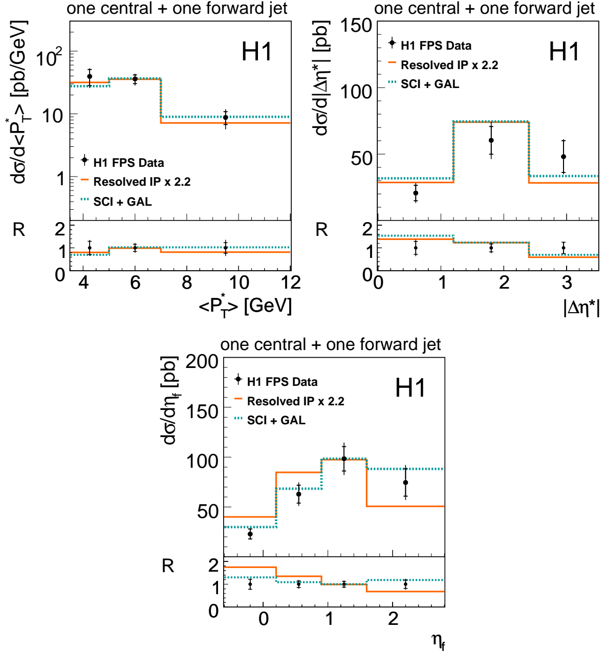
Figure 13: The differential cross section for production of one central and one forward jet shown as a function of the mean transverse momentum of two jets \langle P_T^* \rangle , |\Delta\eta^*| and \eta_f . The inner error bars represent the statistical errors. The outer error bars indicate the statistical and systematic errors added in quadrature. The RP and the SCI+GAL models are shown as solid and dotted lines, respectively. R denotes the ratio of the measured cross sections and MC model predictions to the nominal values of the measured cross sections. The total normalisation error of 6.2% is not shown.
