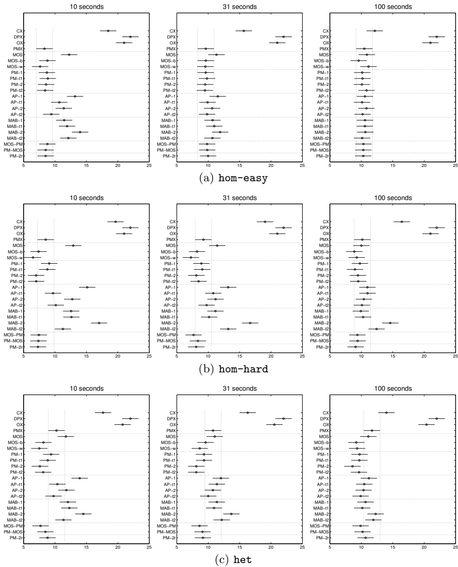
Fig. 1. The ranking performance of different operator selection methods (acronyms see text) with different computation time 10, 31, and 100 seconds on (a) homogeneous easy (b) homogeneous hard or (c) heterogeneous instance set.
