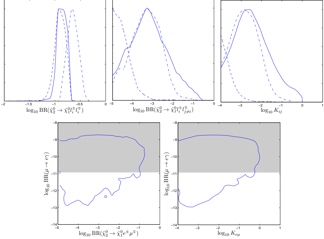
Figure 11: Top left: PDF of \text{BR}(\tilde{\chi}_2^0 \rightarrow l_i l_j \tilde{\chi}_1^0) . Plain, dashed and dash-dotted lines correspond to l_i l_j = ee, \mu\mu, \tau\tau respectively. Top center: PDF of \text{BR}(\tilde{\chi}_2^0 \rightarrow l_i l_j \tilde{\chi}_1^0) . Plain, dashed and dash-dotted lines correspond to l_i l_j = e\mu, e\tau, \mu\tau respectively. Top right: Plain, dashed and dash-dotted lines correspond to K_{e\mu}, K_{e\tau}, K_{\mu\tau} respectively. Bottom: 95% BC region of the joint PDF of \text{BR}(\mu \rightarrow e\gamma) with \text{BR}(\tilde{\chi}_2^0 \rightarrow e\mu\tilde{\chi}_1^0) (left) and K_{e\mu} (right). All of these distributions are for a fixed sign combination at F^T/2R = 1500 GeV, F^Z/M_* = 50 GeV and \tan\beta = 5 . The chosen sign combination represents the typical behaviour of SUSY BRs, while it is somewhat favourable regarding the \text{BR}(\mu \rightarrow e\gamma) constraint.
