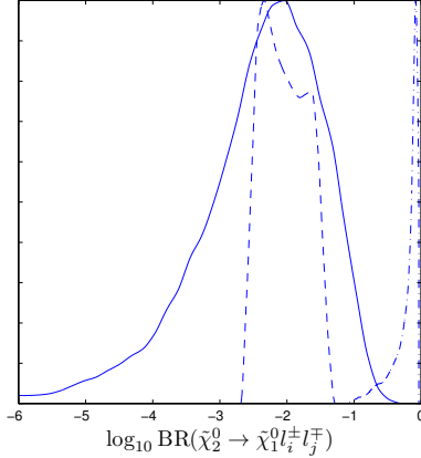
Figure 9: PDFs for \tilde{\chi}_2^0 cascade decays at F^T/2R = 1500 GeV, \tan\beta = 30 and \mathcal{L} = 3 ; dash-dotted line: \text{BR}(\tilde{\chi}_2^0 \rightarrow \tilde{\chi}_1^0 \tau^\pm \tau^\mp) , dashed line: \text{BR}(\tilde{\chi}_2^0 \rightarrow \tilde{\chi}_1^0 \mu^\pm \mu^\mp) , solid line: \text{BR}(\tilde{\chi}_2^0 \rightarrow \tilde{\chi}_1^0 \tau^\pm \mu^\mp) .
