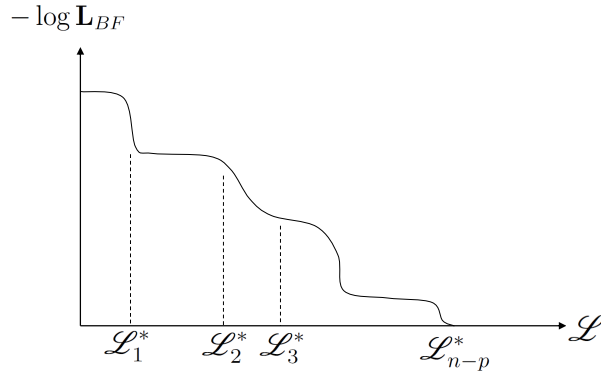
Figure 1: Logarithm of the likelihood of the best fit point, -\log \mathbf{L}_{BF} as a function of \mathcal{L} , for a fit involving n constraints and p parameters. The constraints weaken and eventually decouple as \mathcal{L} increases. The fit becomes perfect, i.e. -\log \mathbf{L}_{BF} = 0 , once only p of the n constraints remain.
