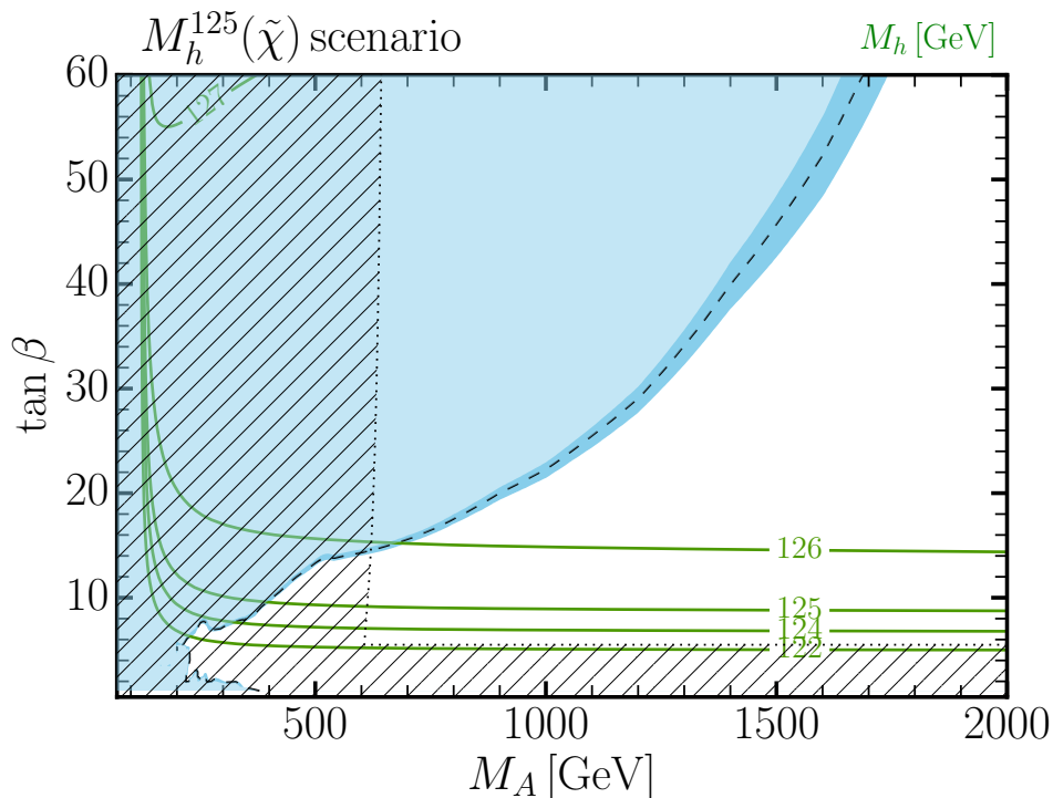
Figure 5: Constraints on the M_h^{125}(\tilde{\chi}) scenario from Higgs searches at the LHC, in the (M_A, \tan \beta) plane. The green solid lines are predictions for the mass of the lighter \mathcal{CP} -even scalar h , the hatched area is excluded by a mismatch between the properties of h and those of the observed Higgs boson, and the blue area is excluded by the searches for additional Higgs bosons (the darker-blue band shows the theoretical uncertainty of the exclusion).
