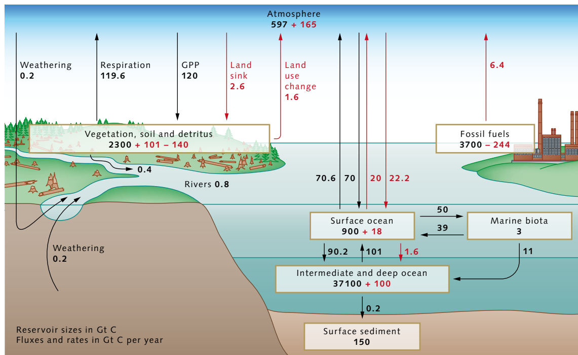
2.1 > The carbon cycle in the 1990s with the sizes of the various reservoirs (in gigatons of carbon, Gt C), as well as the annual fluxes between these. Pre-industrial natural fluxes are shown in black, anthropogenic changes in red. The loss of 140 Gt C in the terrestrial biosphere reflects the cumulative CO 2 emissions from land-use change (primarily slash and burn agricul-
