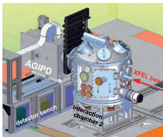
Figure 2 3D view of the second interaction area at the HED instrument of European XFEL: Interaction chamber 2 for DAC and shock experiments. The HIBEF AGIPD 1M detector and the detector bench are shown.
