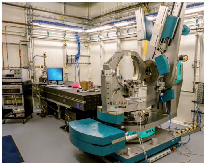
Figure 5 Heavy load diffractometer at the Russian-German beamline P23 at PETRA III.
