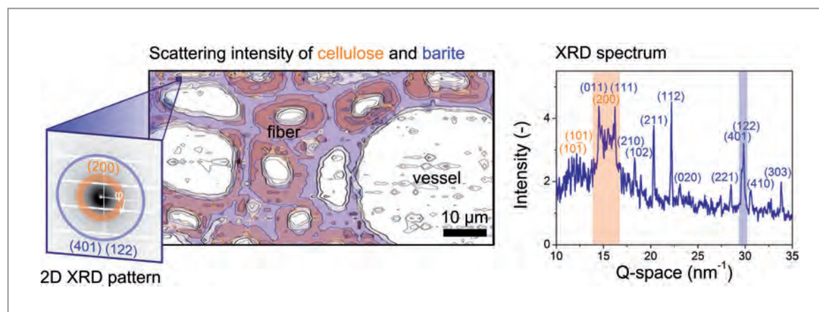
Figure 3 Diffraction enhanced imaging of the distribution of barite ( \text{BaSO}_4 ) inside the cell walls of wood. Each pixel corresponds to the information extracted from individual diffractograms recorded at the same position.
