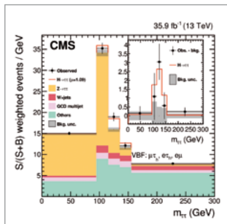
Figure 1 Observed and predicted distribution of the invariant mass of \tau pairs in the CMS analysis of the H \rightarrow \tau\tau decay channel
