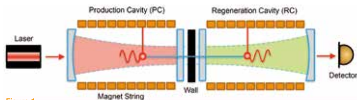
Figure 1 Schematic layout of the ALPS II experiment
