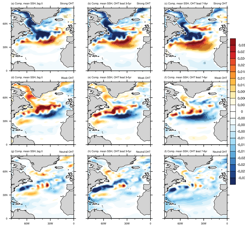
Figure 3.8: Composite mean sea surface height anomalies [m] in ASSIM, related to strong (a-c), weak (d-f), and neutral (g-i) OHT_{50N} phases. I show composites at lag 0 (a,d,g) and composite mean SSH 3-5 (b,e,h) and 7-9 (c,f,i) years after strong and weak OHT_{50N} phases. Stippling indicates significance at the 99% level.
