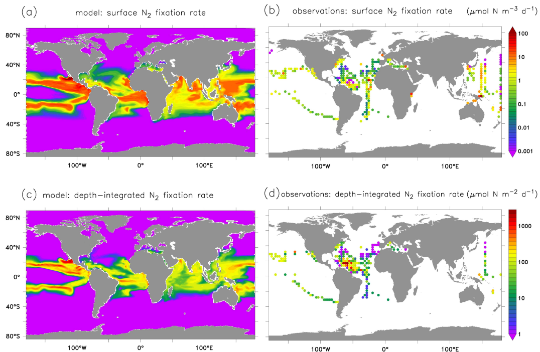
Figure 2.2: Top: Surface N_2 fixation rates ( \mu\text{mol N m}^{-3} \text{d}^{-1} ) (a) in the model (PROG, 100 year mean), and (b) in observations (0–10 m). Bottom: depth-integrated N_2 fixation rates ( \mu\text{mol N m}^{-2} \text{d}^{-1} ) (c) in the model (PROG, 100 year mean) and (d) in observations. Observational data is taken from the database described in Luo et al. (2012), binned on a 3^\circ \times 3^\circ grid. The geometric mean of each bin is shown.
