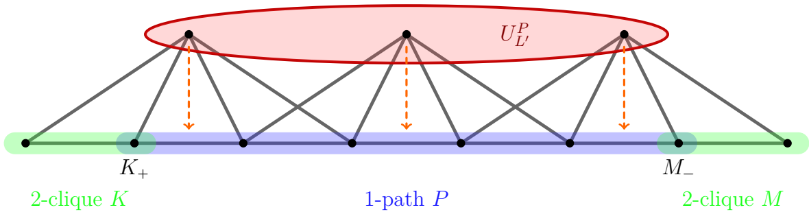
FIGURE 4.1. Building a 2-path Q for k = 1 that connects K and M by adding vertices from U_{L'}^P to a 1-path P connecting K_+ and M_- at the indicated places.
