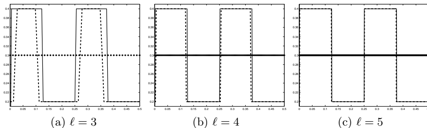
Figure 1: Optimal control \bar{u} (solid) and computed counterpart u_{kh} (dashed) over time after level \ell ( \alpha = k^{4/3} = h^2 ).
