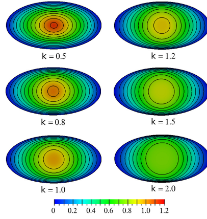
Fig. 7: Solution for ellipse for \varepsilon = 0.1 .
