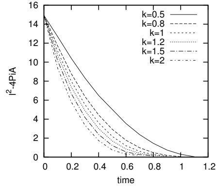
Fig. 10: Isoperimetrical deficit.
