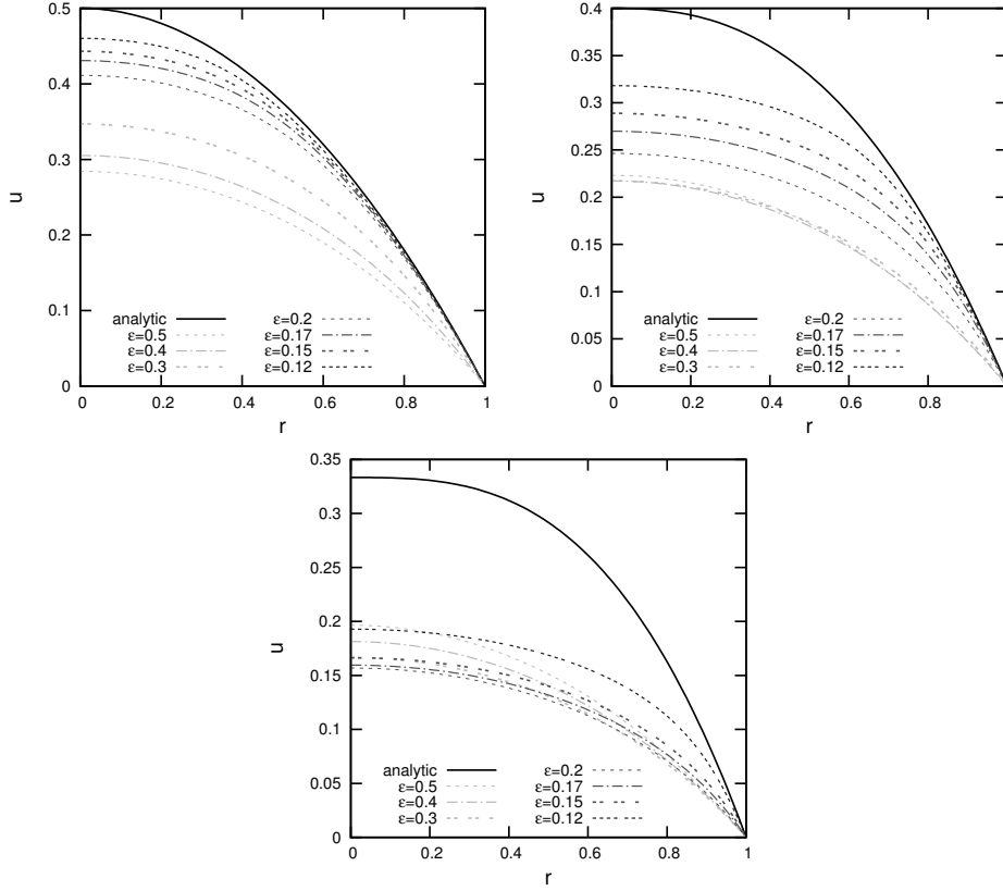
Fig. 5: Radial solution for a circle as initial curve for k = 1, 1.5, 2 .
