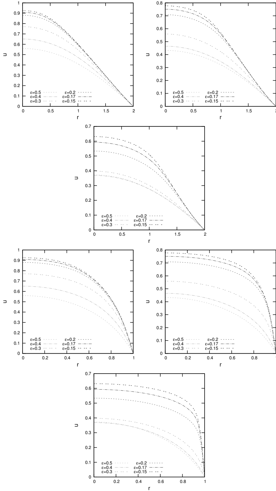
Fig. 6: Solution for ellipse as initial curve. Picture 1–3: Section in direction of the long half axis of the initial curve for k = 1, 1.5, 2 ; Picture 4–6: the same for the short half axis.
