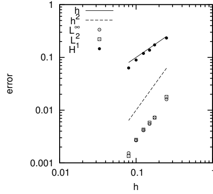
Fig. 1: Discretization error for the unit circle as initial curve where k = 1 , \varepsilon = 0.1 .
