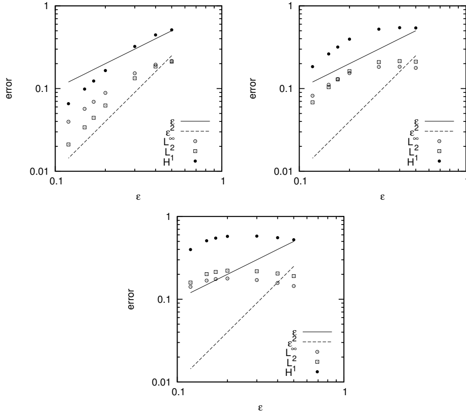
Fig. 3: Regularization error in case of a circle as initial curve for k = 1, 1.5, 2 .
