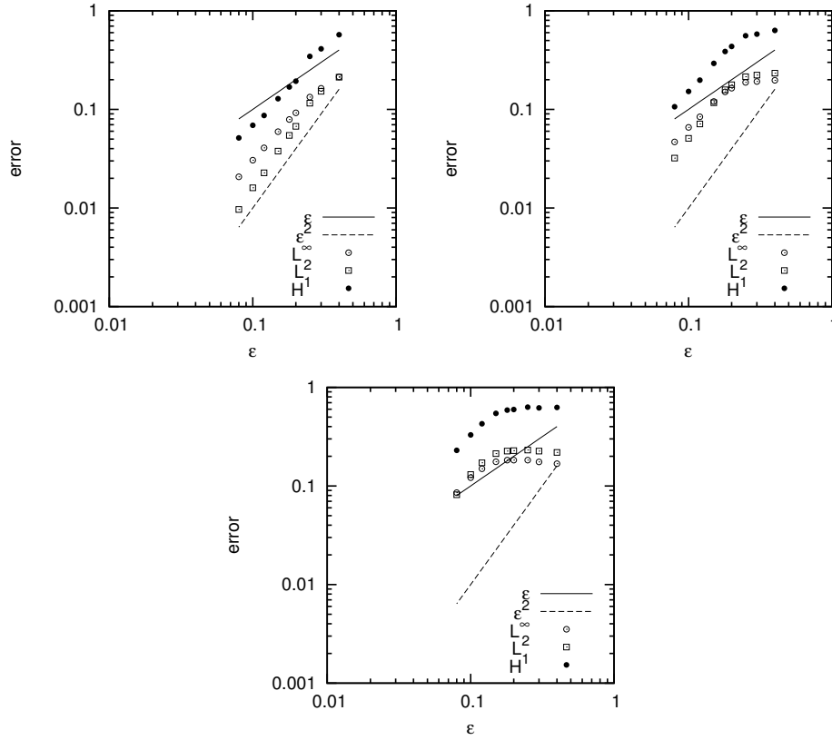
Fig. 8: Total approximation error, \varepsilon = h , for k = 1, 1.5, 2 , in case of a circle as initial curve.
