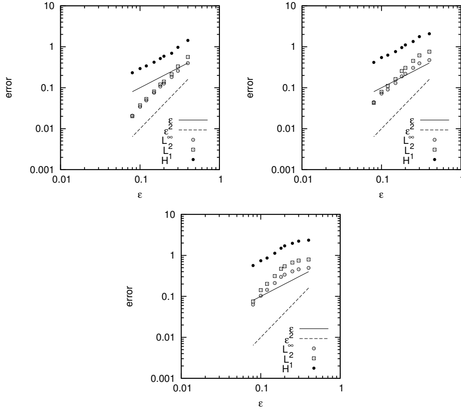
Fig. 9: Total approximation error, \varepsilon = h , for k = 1, 1.5, 2 in case of ellipse with half axes 1 and 2 as initial curve.
