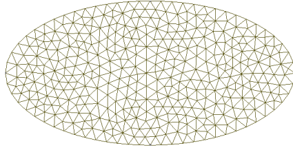
Fig. 11: Mesh for the discretization with size h = 0.15 for ellipse with half axes 1 and 2.
