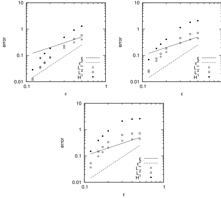
Fig. 4: Regularization error in case of an ellipse as initial curve for k = 1, 1.5, 2 .
