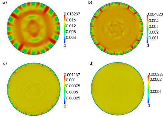
Fig. 2: Discretization error for the unit circle as initial curve (we compare with a discrete solution on a fine grid with size h_0 ). The pictures show the difference u_{h_0}^\epsilon - u_h^\epsilon for \epsilon = 0.09 , k = 1 , h_0 = 0.025 and a) h = 0.4 , b) h = 0.2 , c) h = 0.1 , d) h = 0.05 .
