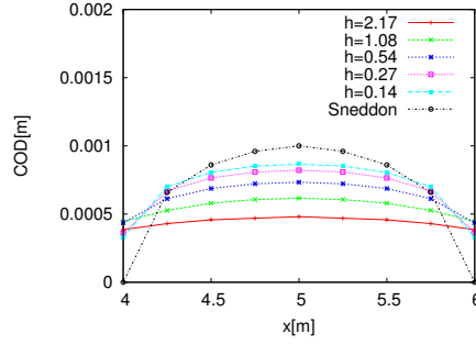
Figure 16: Example 4: COD for different h . Sneddon's black line line corresponds to his analytical 3D solution.
