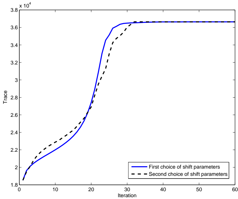
Fig. 2 Monotonicity of ADI iteration: convection-diffusion equation with the space dimension n = 4900
